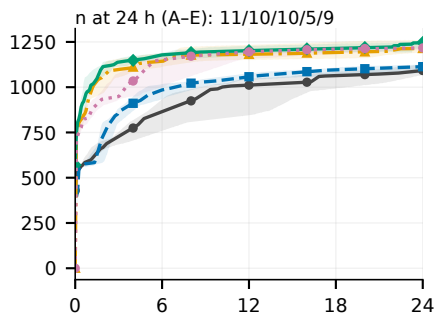
(g) Kamailio
