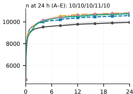
(g) Kamailio
