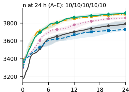
(h) Forked-daapd
