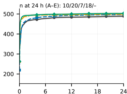
(e) Exim
