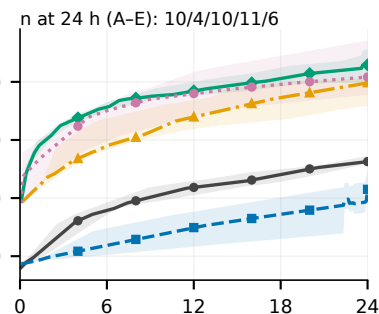
(h) Forked-daapd
