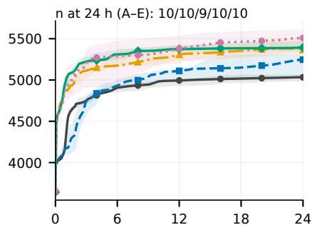
(f) Live555
