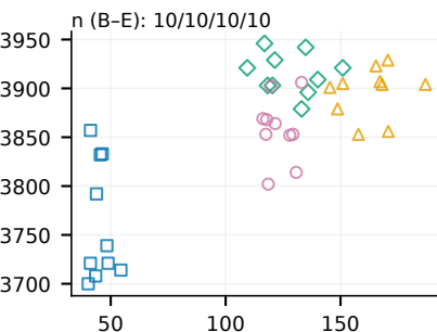
(h) Forked-daapd
