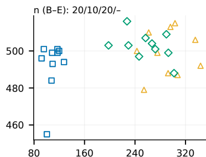
(e) Exim
