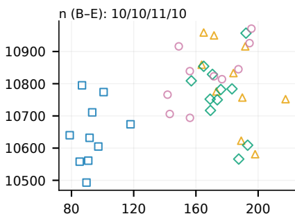
(g) Kamailio
