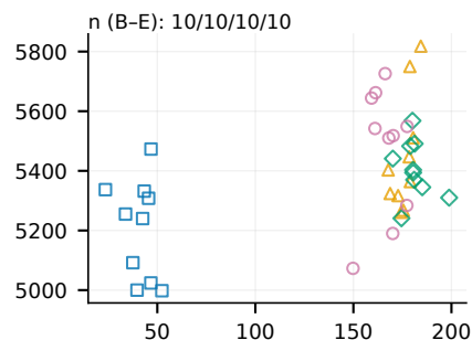
(f) Live555
