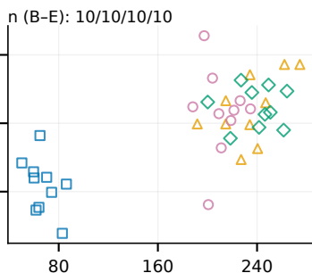
(g) Kamailio
