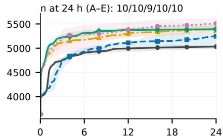
(f) Live555
