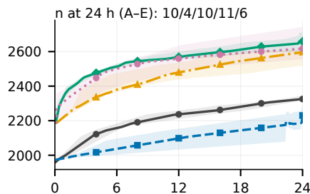
(h) Forked-daapd
