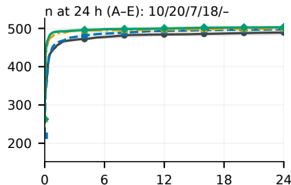
(e) Exim
