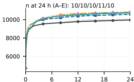
(g) Kamailio
