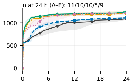
(g) Kamailio
