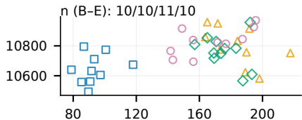
(g) Kamailio
