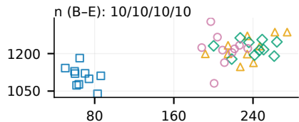
(g) Kamailio
