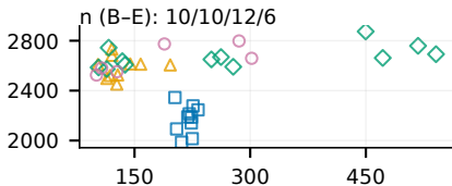
(h) Forked-daapd
