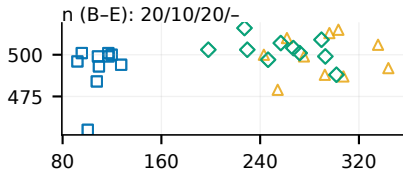
(e) Exim
