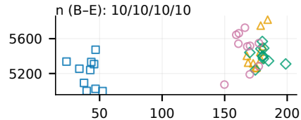
(f) Live555
