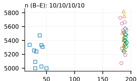
(f) Live555
