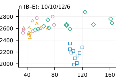
(h) Forked-daapd
