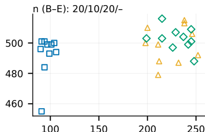
(e) Exim
