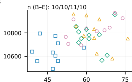
(g) Kamailio
