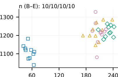
(g) Kamailio
