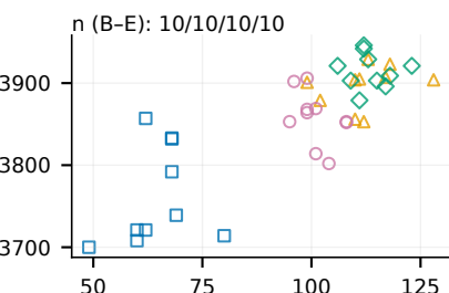
(h) Forked-daapd
