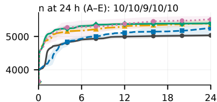
(f) Live555
