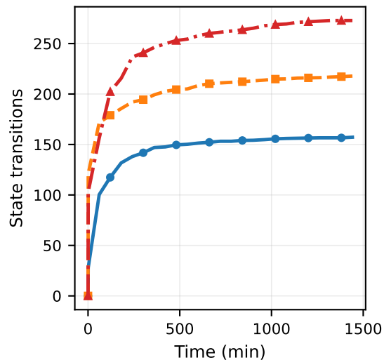
Forked-daapd
