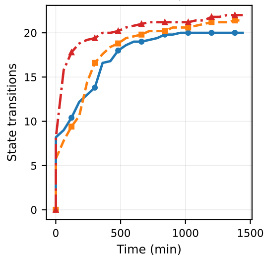
Forked-daapd
