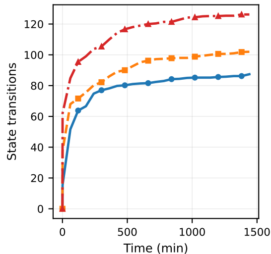
Mosquitto
