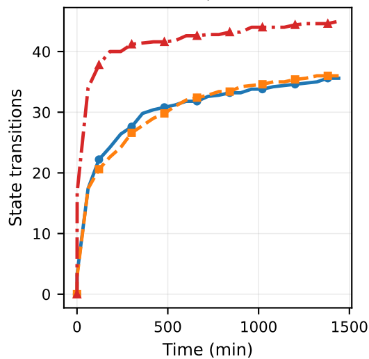
Mosquitto
