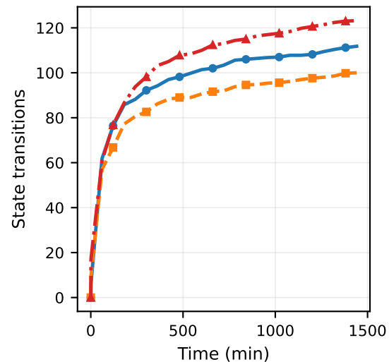
Kamailio
