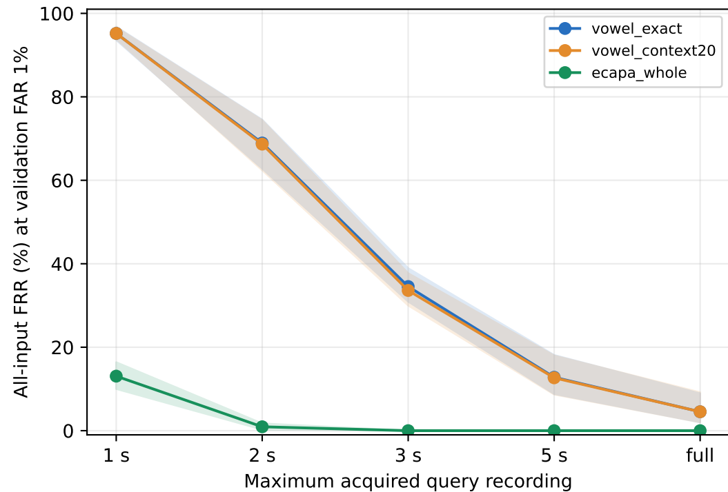
test-native-n10-verification; 95% speaker bootstrap
