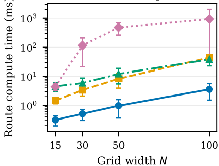
(b) Decision computation
