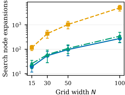
(c) Classical search work
