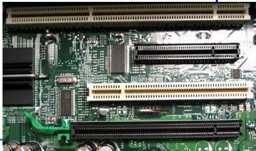
PCI-X (64bit)
