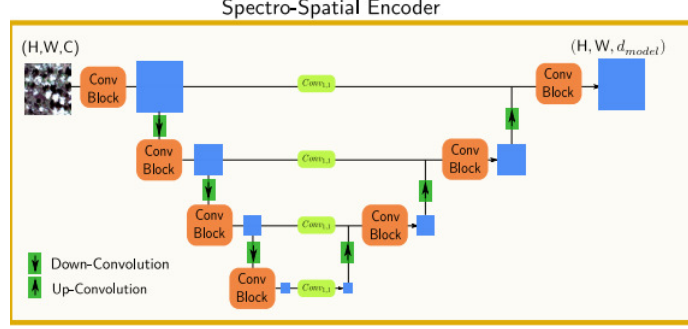
Fig. 2 U-BARN Architecture
