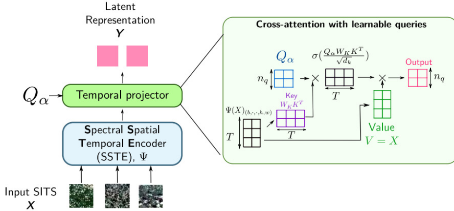
Fig. 3 ALISE Architecture
