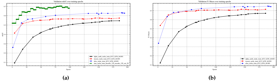
Fig. 8 Increasing trends of the validation F1 Macro (Fig. 8b) and mIoU (Fig. 8a) metrics during training (validation fold). As shows Fig. 8a, U-TAE is trained only for 100 epochs. Fig. 8b does not show the U-TAE curve as the original implementation does not log the F1 Macro metric during training.
