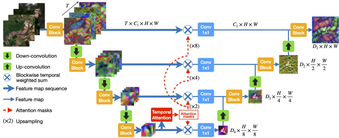
Fig. 4 U-TAE Architecture
