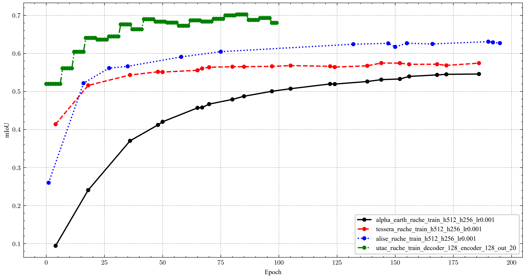
Validation mIoU over training epochs
