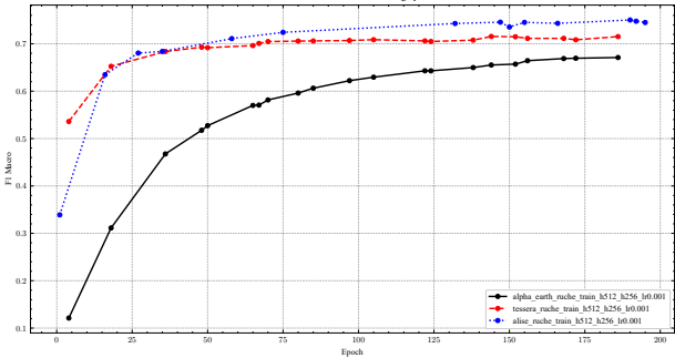
Validation F1 Macro over training epochs
