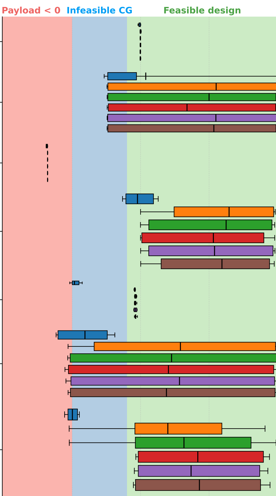
e) Cargo aircraft with 2040 technology projections
