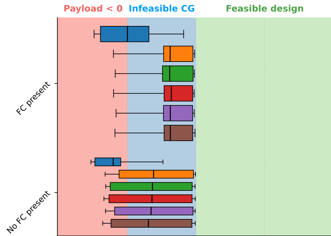
a) Passenger aircraft with 2030 technology projections
