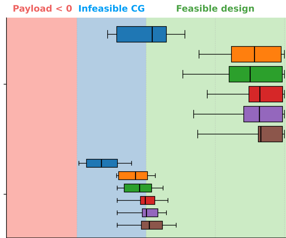
c) Passenger aircraft with 2050 technology projections
