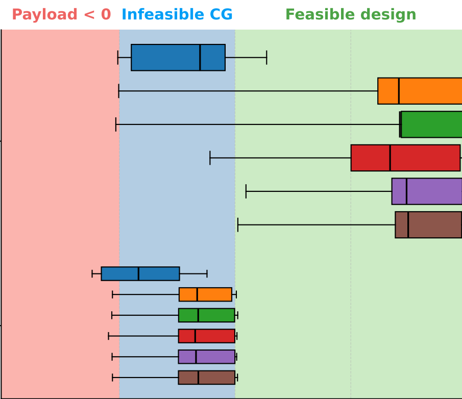
b) Passenger aircraft with 2040 technology projections
