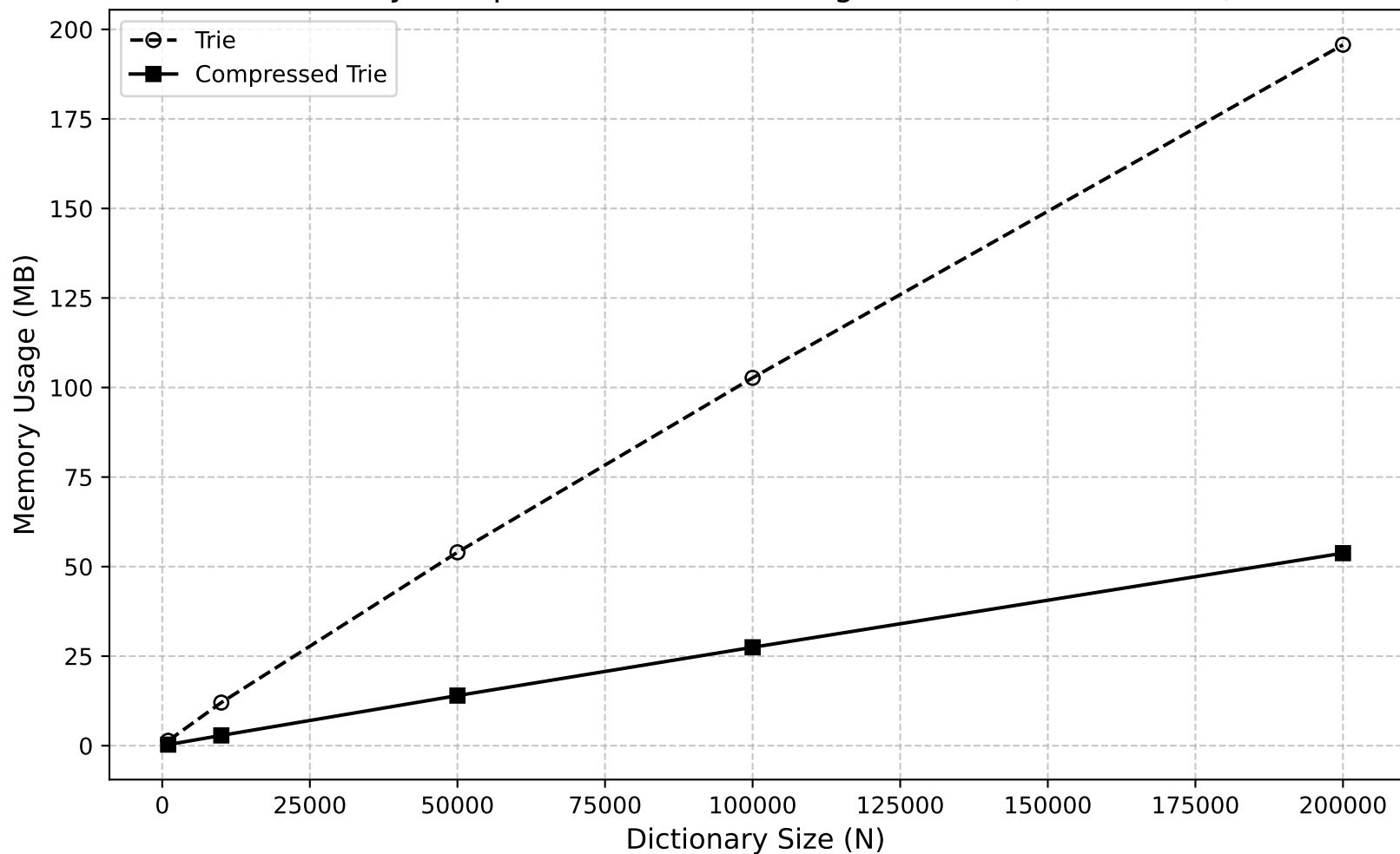
Memory Comparison: Variable Length Words (Normal Dist.)
