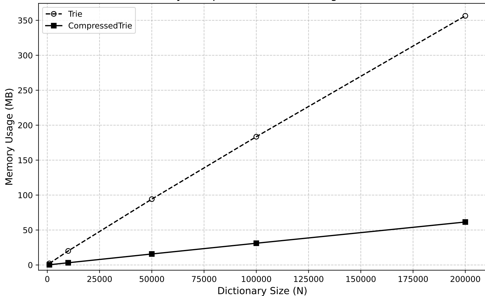
Memory Comparison: Variable Length Words
