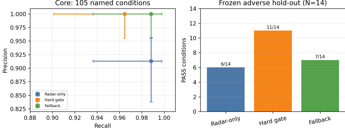
Fig. 1. Frozen named-condition evidence. Left: core precision-recall and descriptive Wilson intervals. Right: system PASS on the 14-condition adverse hold-out. Neither grid estimates road prevalence.
