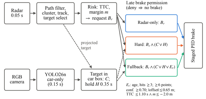
Fig. 1. Shared sensor-to-brake pipeline. All policies receive the same radar request B_r and car-only confirmation C /hold H and differ only in late permission: hard gating denies B_r without a car box at the projected target; fallback also grants it when the emergency condition E_r holds.
