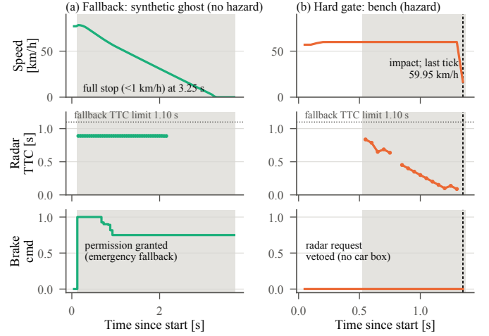
Fig. 2. Frozen tick logs. (a) Fallback, six-point synthetic ghost: emergency permission at 0.15 s and a full stop. (b) Hard gate, hold-out bench: the radar request is vetoed until impact (dashed). Grey: radar request B_r present. Selection: the run whose severity descriptors equal the policy median (ghost onset speed, duration, and peak deceleration over 20 runs; bench pre-impact speed over five runs), lowest scenario/run identifier on ties.
