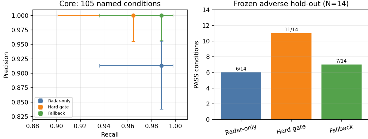
Fig. 1. Frozen named-condition evidence. Left: core precision-recall with descriptive Wilson ranges on constructed named conditions. Right: system PASS on the 14-condition adverse hold-out. Neither grid estimates road prevalence.
