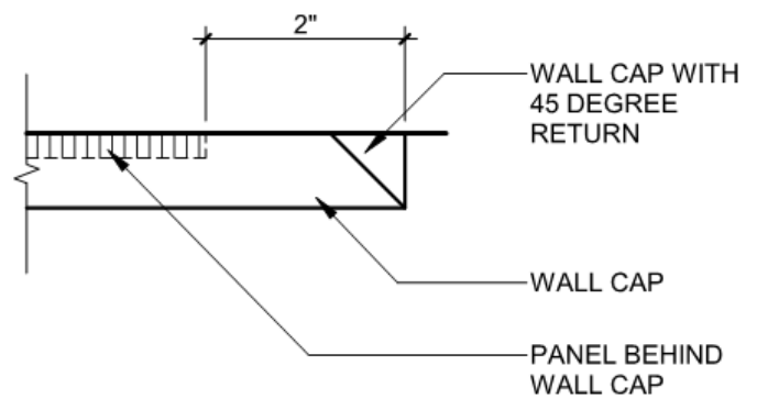
3 WP-3 PLAN 6" = 1'-0"
