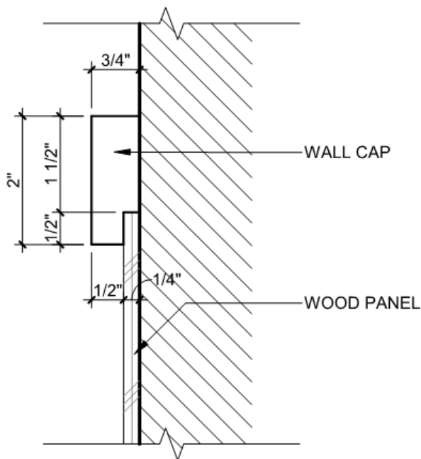
1 WP-3 SECTION 6" = 1'-0"
