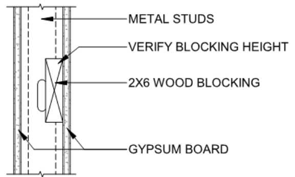
2 BLKG-2 1 1/2" = 1'-0" 2x WOOD BLOCKING
