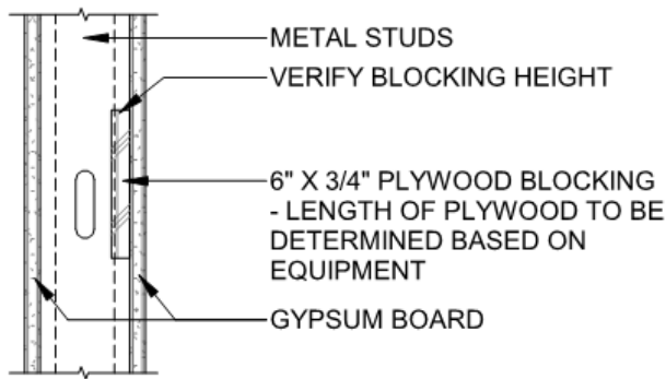
1 BLKG-2 1 1/2" = 1'-0" PLYWOOD BLOCKING
