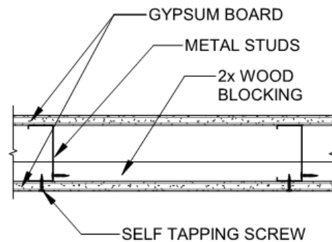
4 BLKG-2 1 1/2" = 1'-0" 2x WOOD BLOCKING
