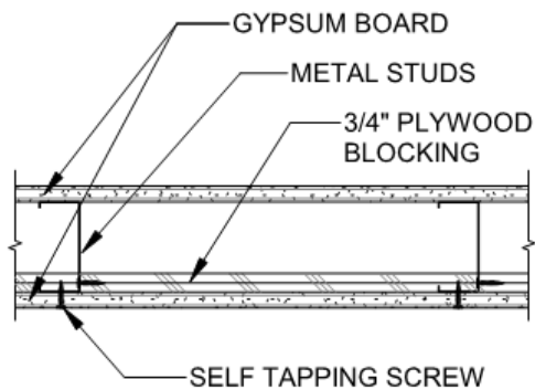
3 BLKG-2 1 1/2" = 1'-0" PLYWOOD BLOCKING
