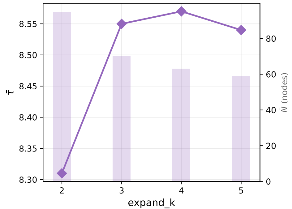
HumanEval
