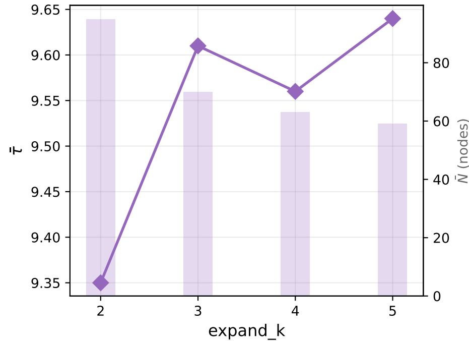
MATH-500
