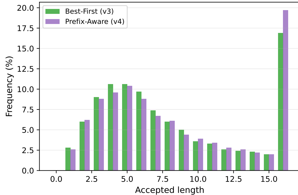
HumanEval
