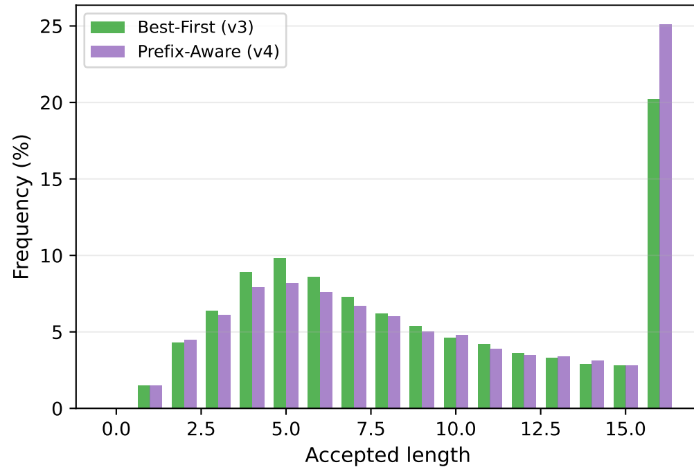
MATH-500
