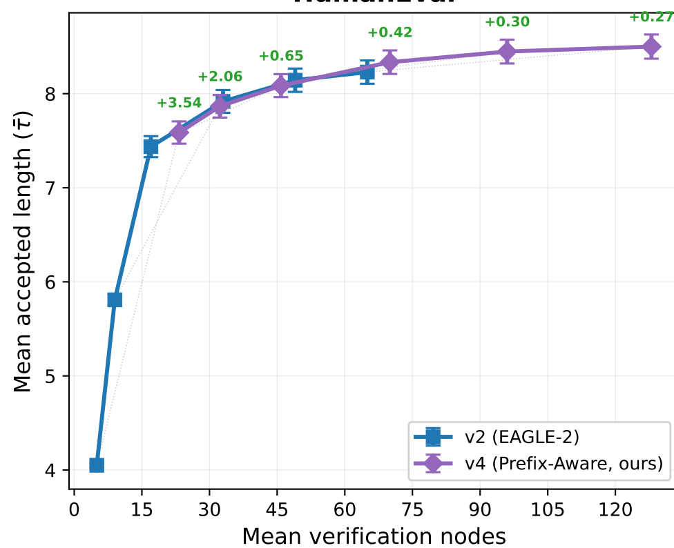
HumanEval
