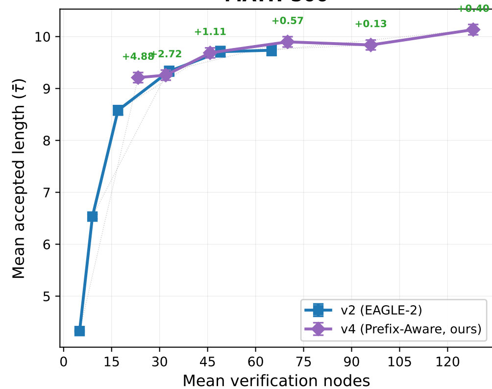
MATH-500
