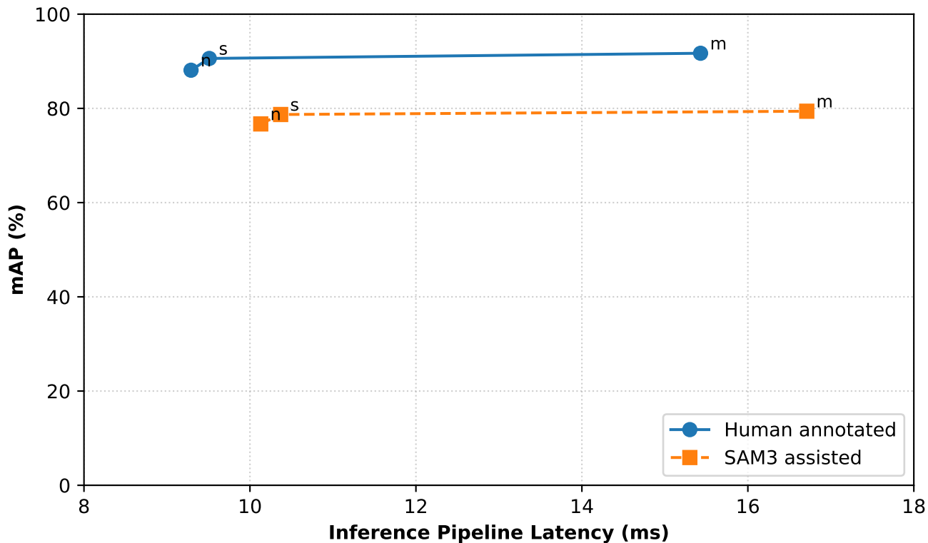
YOLOv8 Performance: Human vs. SAM 3 Annotation
