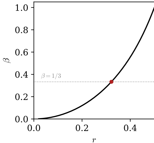
(c) \beta = \log m / \log(2/m)
