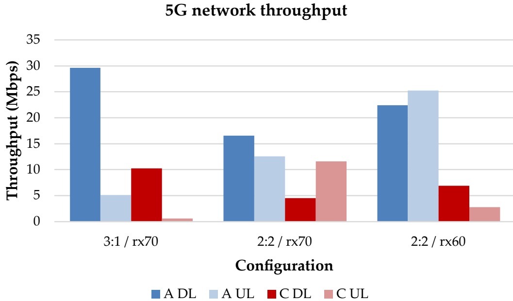
Figure 6.7: TCP throughput at Locations A (2 m) and C (10 m) across the three 5G rounds. The x-axis shows the specific configuration used in each round.
