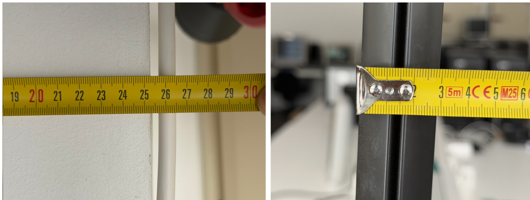
Figure 5.8: Tape measured thickness readings for the two obstructions on the direct path: the concrete wall at Location C (25.3 cm) and the office partition at Location B (3 cm).
