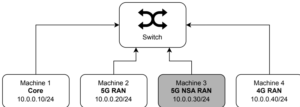
Figure 4.1: Network topology of the four machines, showing the role of each machine and its static IP address. The machine in gray was not used in the actual testbed, but was reserved for a 5G NSA deployment.
