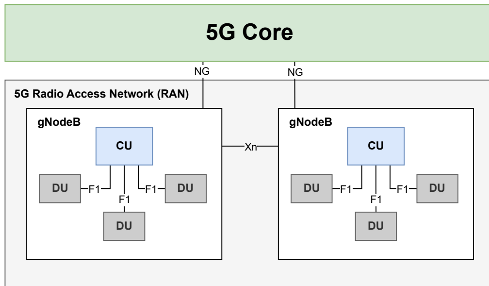
Figure 2.6: 5G RAN [35]
