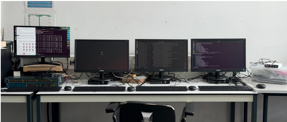
Figure 4.2: The bench, showing all 4 machines. From left to right: 4G RAN, 5G NSA (unused), Core and 5G RAN. Connected to the 4G RAN machine is the bladeRF xA4, and on the rightmost side, connected to the 5G RAN machine, is the NI B2901.
