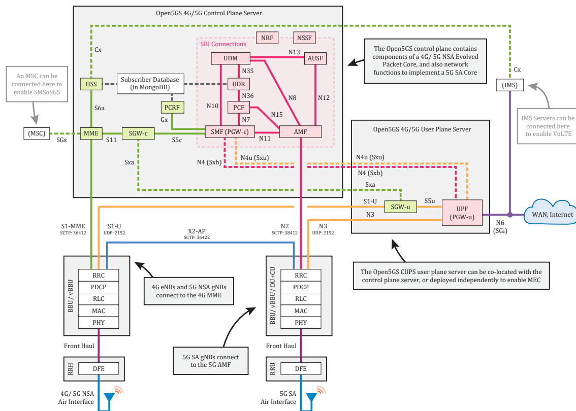
Figure 2.1: 5G Network architecture diagram from the Open5GS project [16]. Used under the AGPL-3.0 license.
