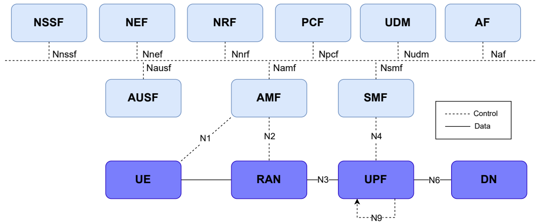
Figure 2.9: 5G Core Network Architecture [18]
