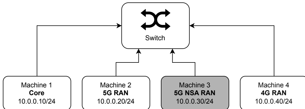
Figure 5.1: Network topology of the four machines, showing the role of each machine and its static IP address. The machine in gray was not used in the actual testbed, but was reserved for a 5G NSA deployment.
