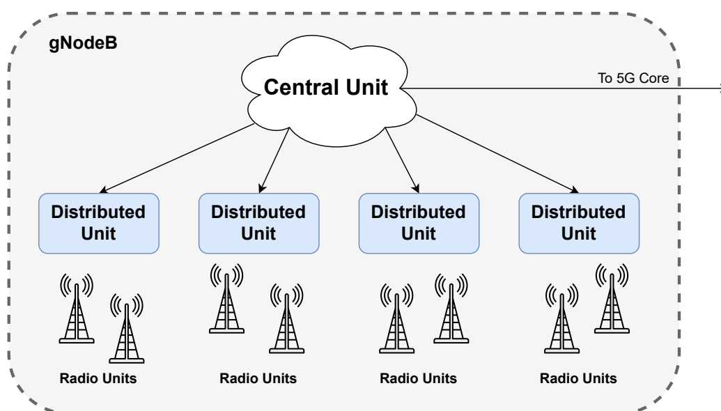
Figure 2.4: gNodeB Architecture [24]
