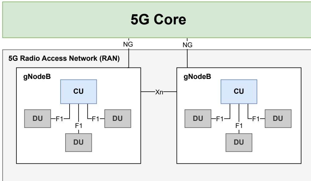
Figure 2.6: 5G RAN [24]
