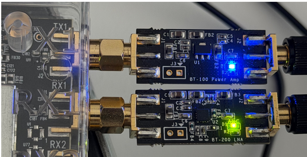
Figure 4.5: The BT-200 LNA and BT-100 power amplifier bias tees, mounted on the bladeRF xA4's RX1 and TX1 ports respectively.
