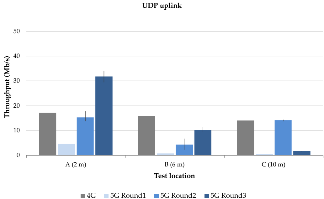
Figure 6.4: UDP uplink throughput at each test location, throughout the three rounds of testing. The black lines represent the range between Min/Max throughput values between each repetition for that combination.
