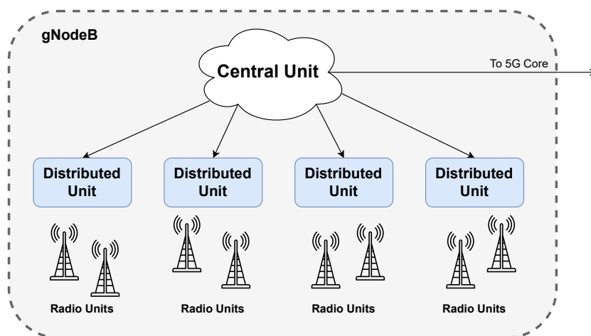
Figure 2.4: gNodeB Architecture [36].
