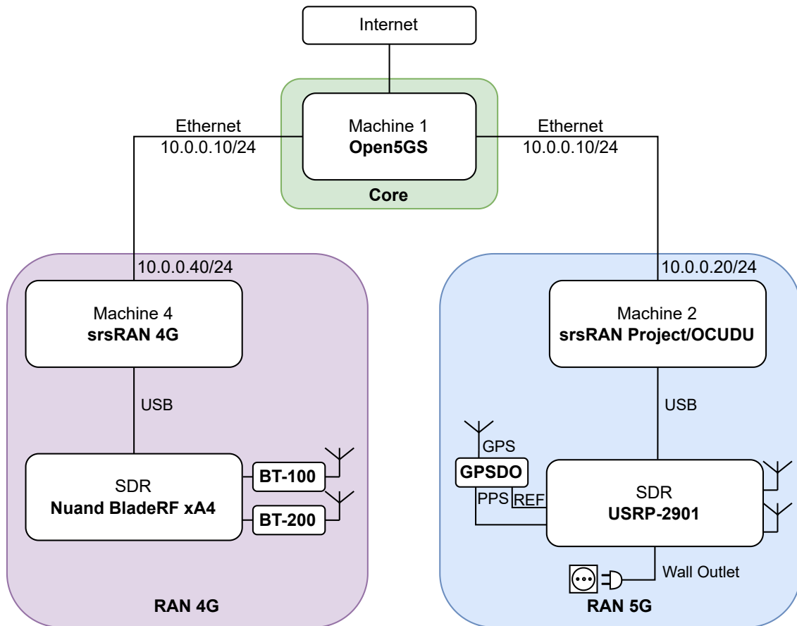
Figure 4.6: The testbed as deployed: the Open5GS core on Machine 1, the 5G RAN on Machine 2 with the USRP-2901 and the GPSDO, and the 4G RAN on Machine 4 with the bladeRF xA4 and its BT-100/BT-200 front-end. The unused 5G NSA machine, the Ethernet switch and the UE are not shown.
