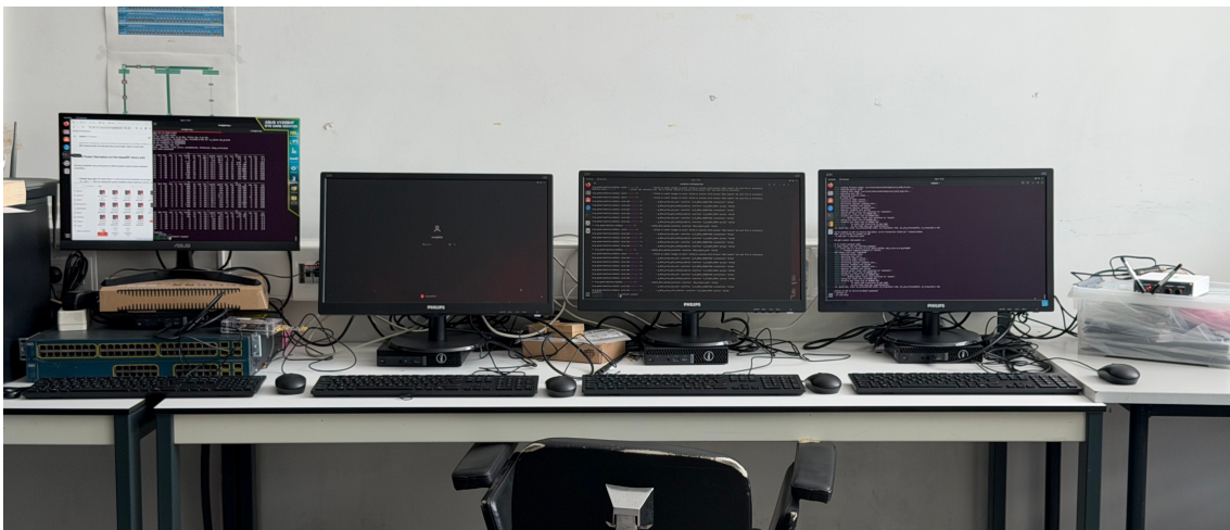
Figure 4.2: The bench, showing all four machines. From left to right: 4G RAN (unused), Core, and 5G RAN. Connected to the 4G RAN machine is the bladeRF xA4, and connected to the 5G RAN machine is the USRP-2901.
