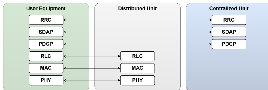
Figure 2.5: 5G RAN Protocol Stack across the three types of units [36].
