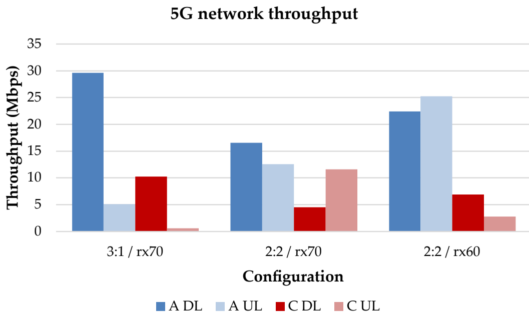
Figure 6.7: TCP throughput at Locations A (2 m) and C (10 m) across the three 5G rounds, labeled by the configuration tested in each location.
