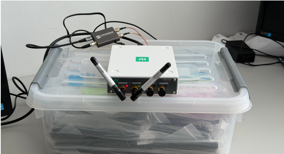
Figure 5.4: The B2901 and the Leo Bodnar GPSDO, as connected on the bench.
