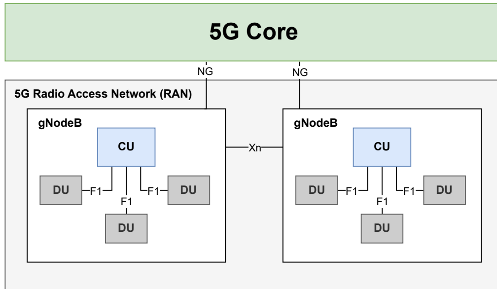
Figure 2.6: 5G RAN [33]
