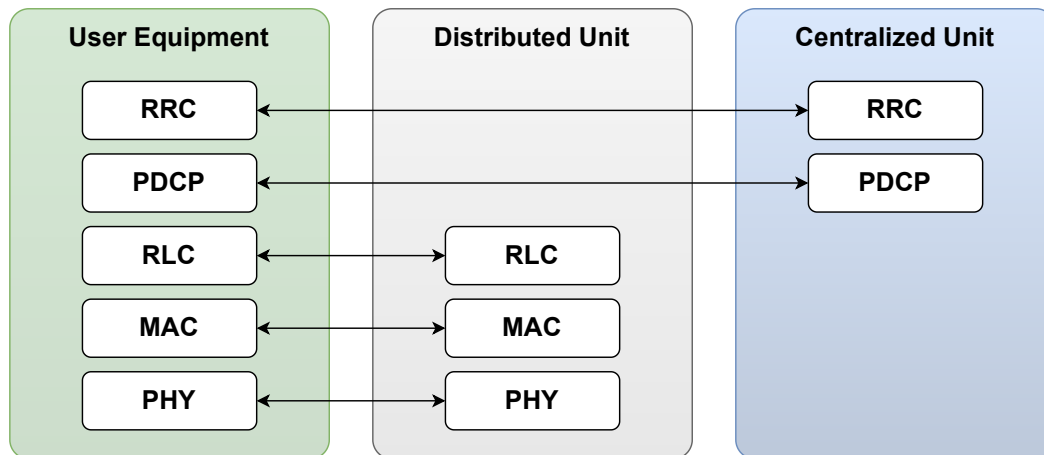
Figure 2.5: 5G RAN Protocol Stack [33]
