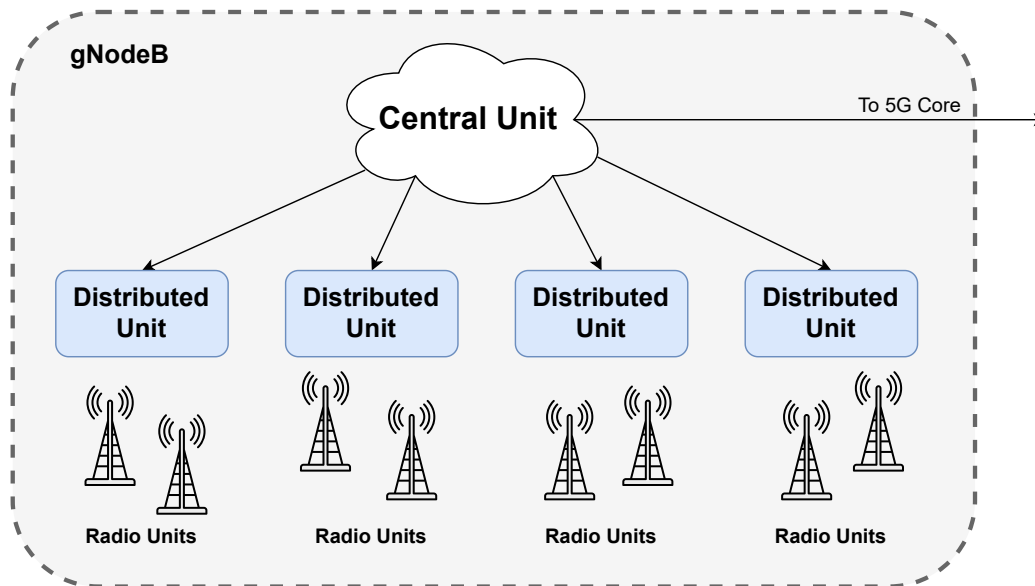
Figure 2.4: gNodeB Architecture [33]
