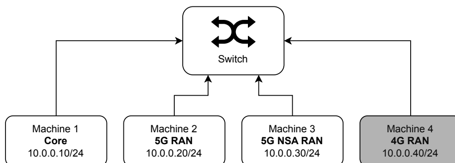
Figure 5.1: Network topology of the four machines, showing the role of each machine and its static IP address.
