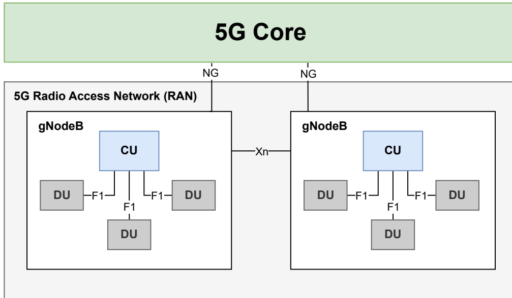
Figure 2.6: 5G RAN [23]
