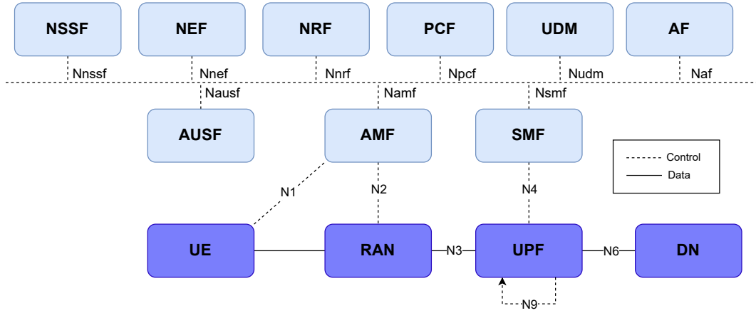
Figure 2.9: 5G Core Network Architecture [23]
