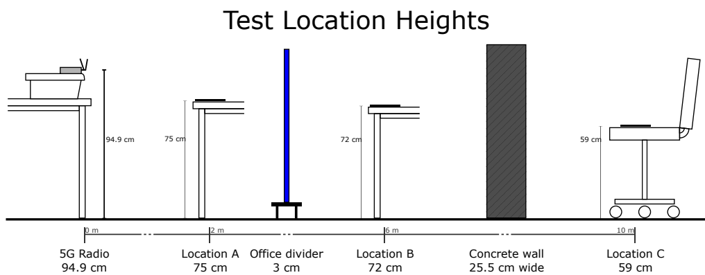
Figure 5.5: Elevation view showing the mounting height of the radio and the UE height at each test location, along with the obstruction on the path to locations B and C.
