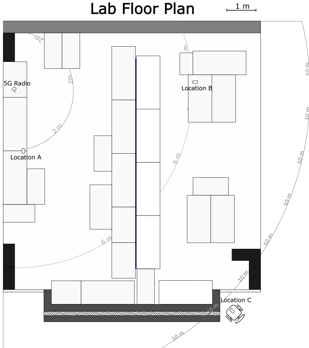
Figure 5.4: Plan view of the room, showing the radio position and the three UE test locations, drawn to scale.
