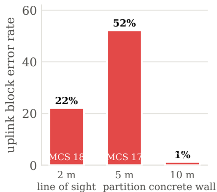
...but only the far point actually decodes
