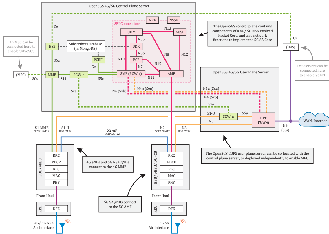
Figure 2.1: 5G Network architecture diagram from the Open5GS project [25]. Used under the AGPL-3.0 license.
