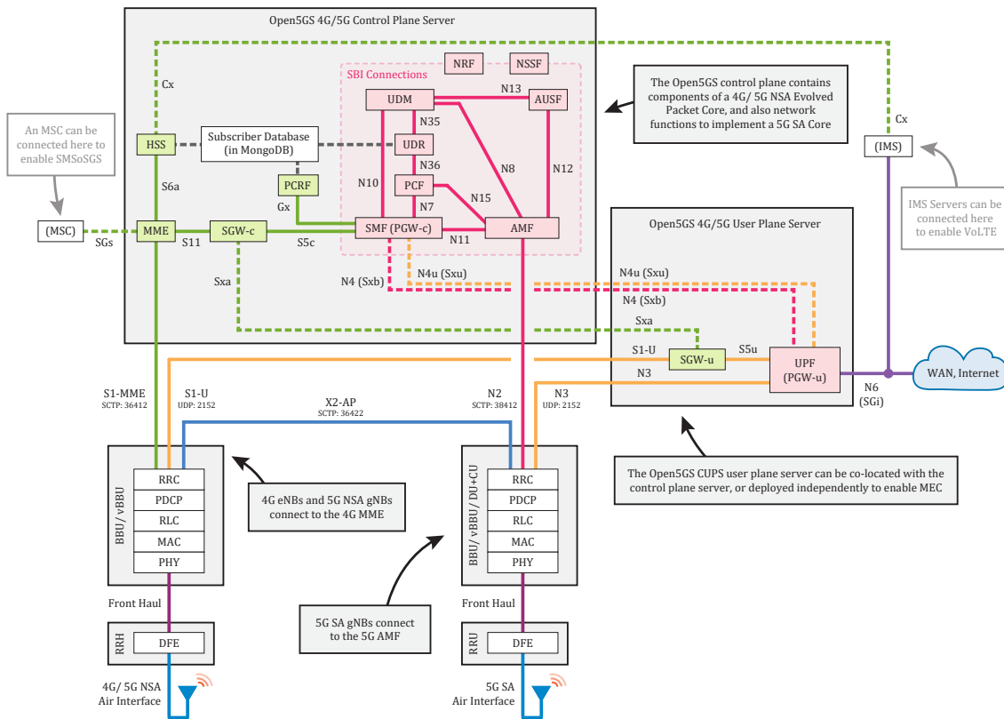
Figure 2.1: 5G Network architecture diagram from the Open5GS project [20]. Used under the AGPL-3.0 license.
