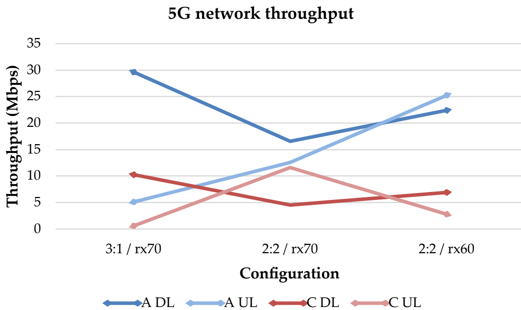
Figure 6.5: TCP throughput at Locations A (2m) and C (10m) across the three 5G configurations. Exactly one parameter changes at each step: the TDD pattern between the first two points, with rx_gain held at 70, and rx_gain between the last two, with the 2:2 pattern held fixed. Location B is omitted because its Round 2 data was discarded (Section 5.2.2). The first configuration was measured once per condition ( n=1 ); the other two use three repetitions.
