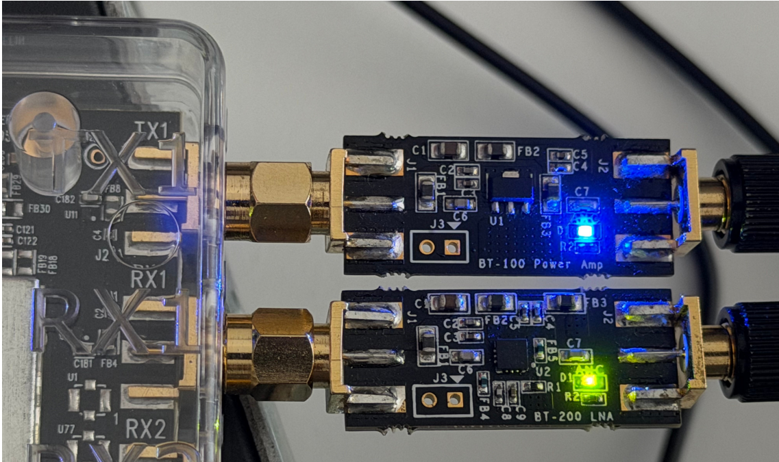
Figure 4.5: The BT-200 LNA and BT-100 power amplifier bias tees, mounted on the bladeRF xA4’s RX1 and TX1 ports respectively.
