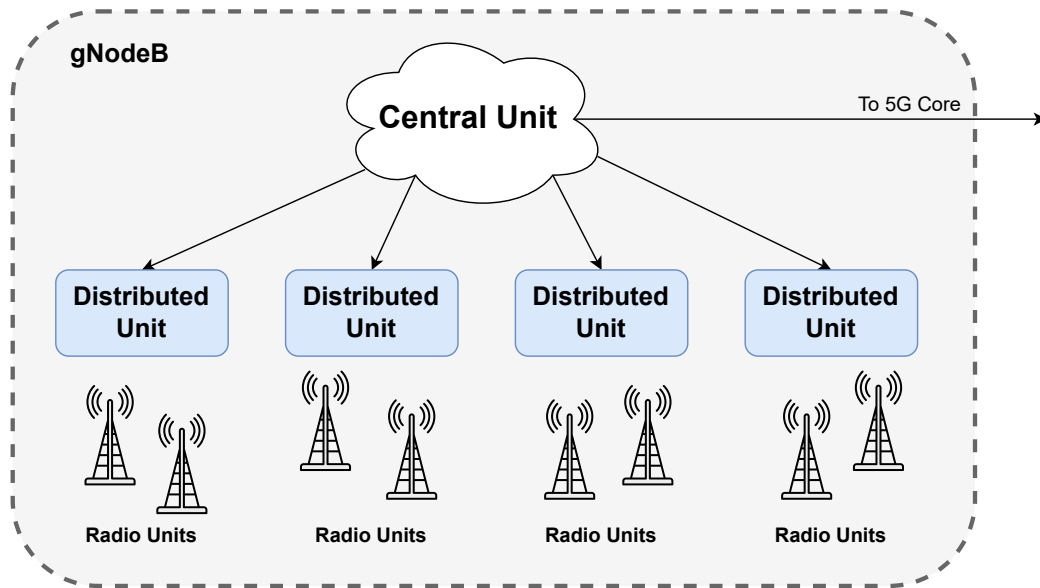
Figure 2.4: gNodeB Architecture [32]
