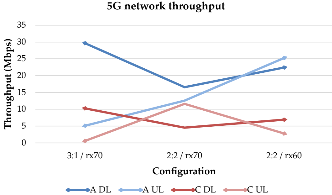
Figure 6.5: TCP throughput at Locations A (2 m) and C (10 m) across the three 5G configurations. Exactly one parameter changes at each step: the TDD pattern between the first two points, with rx_gain held at 70, and rx_gain between the last two, with the 2:2 pattern held fixed. Location B is omitted because its Round 2 data was discarded (Section 5.2.2). The first configuration was measured once per condition ( n=1 ); the other two use three repetitions.
