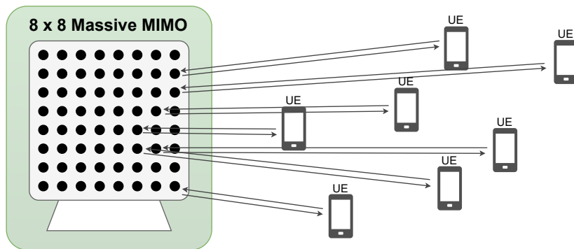
Figure 2.7: Example of a massive MIMO, in which one array of antennas serves several UEs on the same time-frequency resources.
