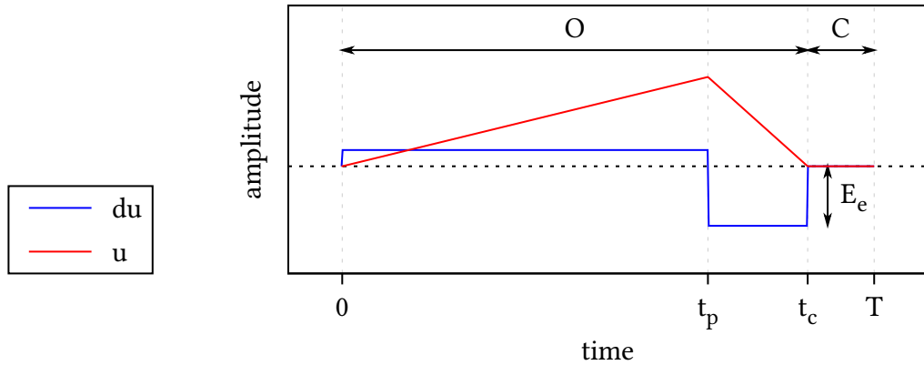
Figure 18 | The triangular pulse model for u'_\Delta(t) (blue) and u_\Delta(t) (red) during a single period of length T . The parameters used in this model are identical to Figure 16, except for the lack of a return phase and that the ‘instant’ of maximum excitation t_e now spans the interval [t_p, t_c] .
