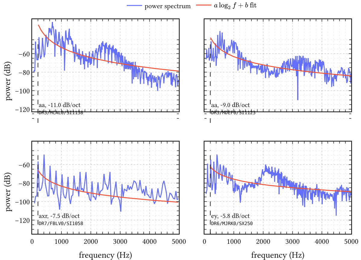
Figure 47 | Example of spectral tilt fits on TIMIT vowel segments. Each panel shows the empirical power spectrum together with the fitted trend a \log_2 f + b . The dashed vertical line marks the 200 Hz cutoff above which the fit is performed. The four examples span a representative range from steeper to flatter observed rolloff.
