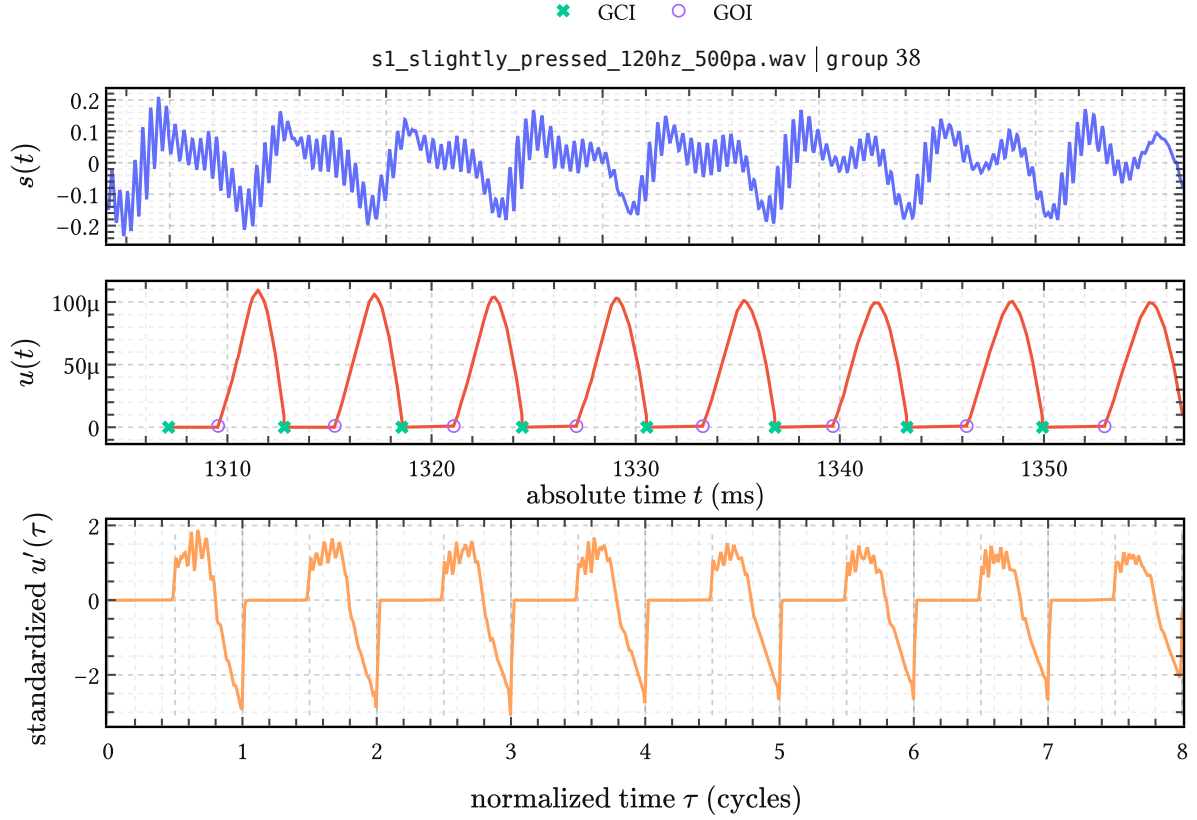
Figure 41 | Registration of one EGIFA voiced group. Top: raw speech s(t) in physical time. Middle: raw glottal flow u(t) with LBGID-detected GCI and GOI landmarks. Bottom: the group after differentiation, normalization, and warp to normalized time \tau , shown as u'(\tau) ; GCIs at integers, GOIs at half-integers.
