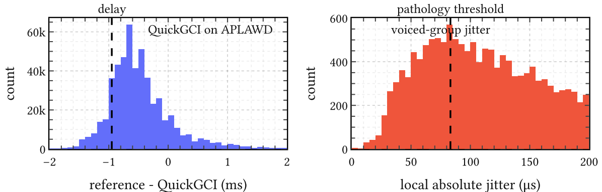
Figure 45 | Two APLAWD diagnostics. Left: QuickGCI timing errors against the hand-corrected GCI references. The mode is centered close to the expected larynx-to-microphone delay. Right: local absolute jitter measured over retained voiced groups. Most of the mass lies well below the usual pathology threshold.
