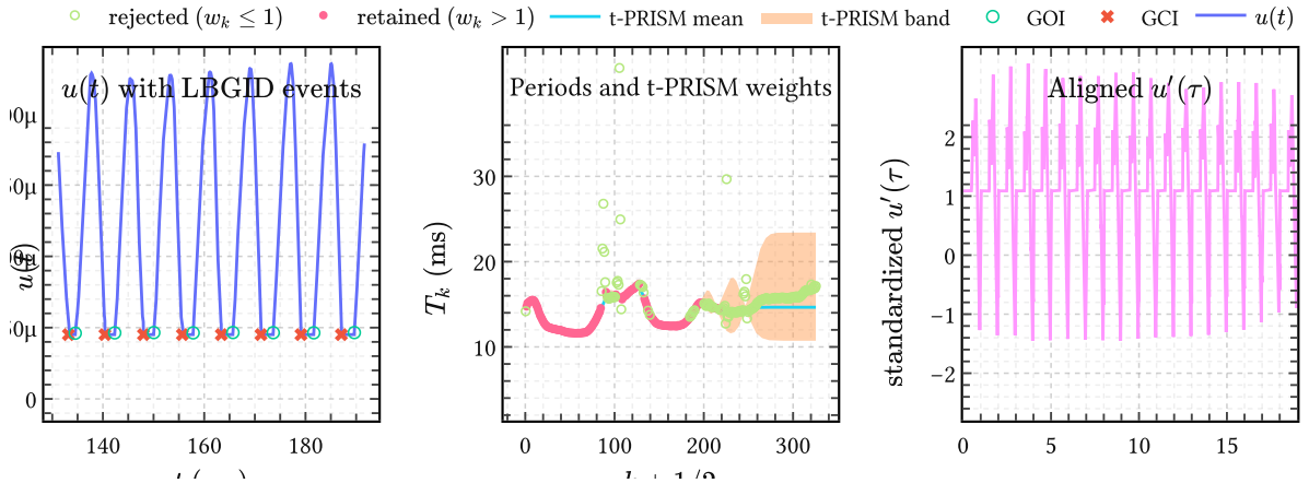
Figure 42 | The EGIFA registration pipeline on one recording. (a) Raw glottal flow with LBGID GCI and GOI events. (b) Implied period sequence over the full recording; t-PRISM posterior mean and uncertainty band with retained inliers. (c) One retained voiced group in shared cycle time \tau after smoothing, differentiation, GOI-aware registration, and per-group normalization.
