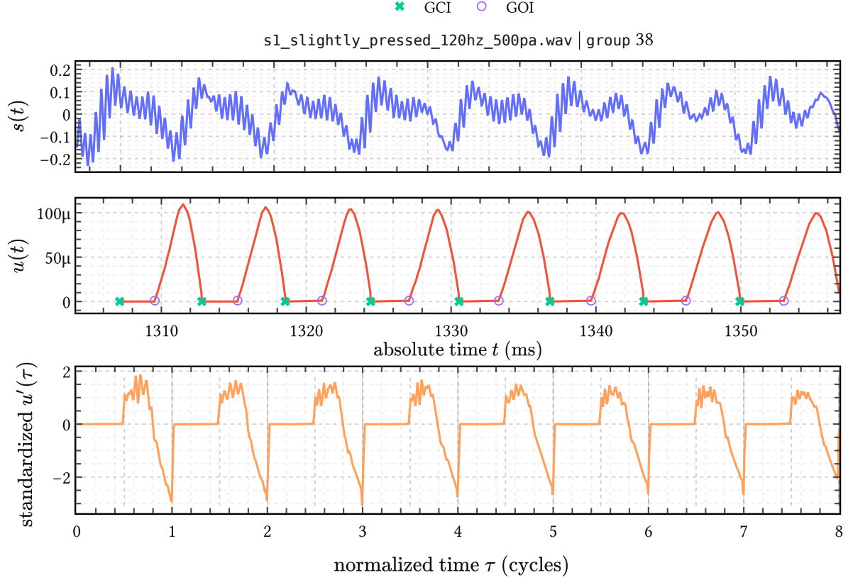
Figure 34 | Registration of one EGIFA voiced group. Top: raw speech s(t) in physical time. Middle: raw glottal flow u(t) with LBGID-detected GCI and GOI landmarks. Bottom: the group after differentiation, normalization, and warp to normalized time \tau , shown as u'(\tau) ; GCIs at integers, GOIs at half-integers.
