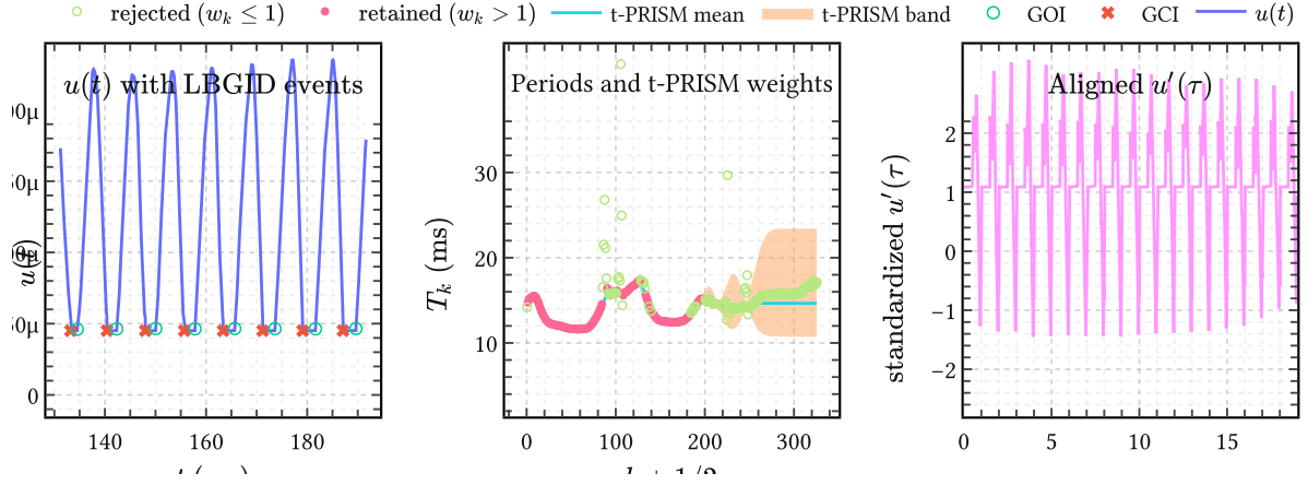
Figure 35 | The EGIFA registration pipeline on one recording. (a) Raw glottal flow with LBGID GCI and GOI events. (b) Implied period sequence over the full recording; t-PRISM posterior mean and uncertainty band with retained inliers. (c) One retained voiced group in shared cycle time \tau after smoothing, differentiation, GOI-aware registration, and per-group normalization.
