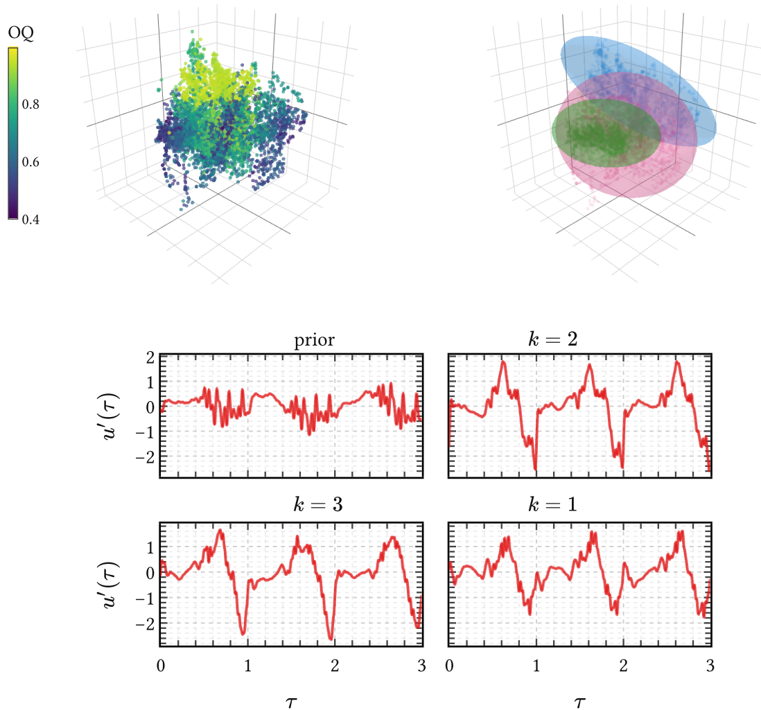
Figure 30 | g-QPACK surrogate: manifold space, quantization, and data-space samples. Same three-step layout as Figure 28, but here the fitted quantization uses only K = 3 components. The GOI-aware gate suppresses open-phase variance structurally; compare the tighter bottom-row waveform spread with Figure 28.
