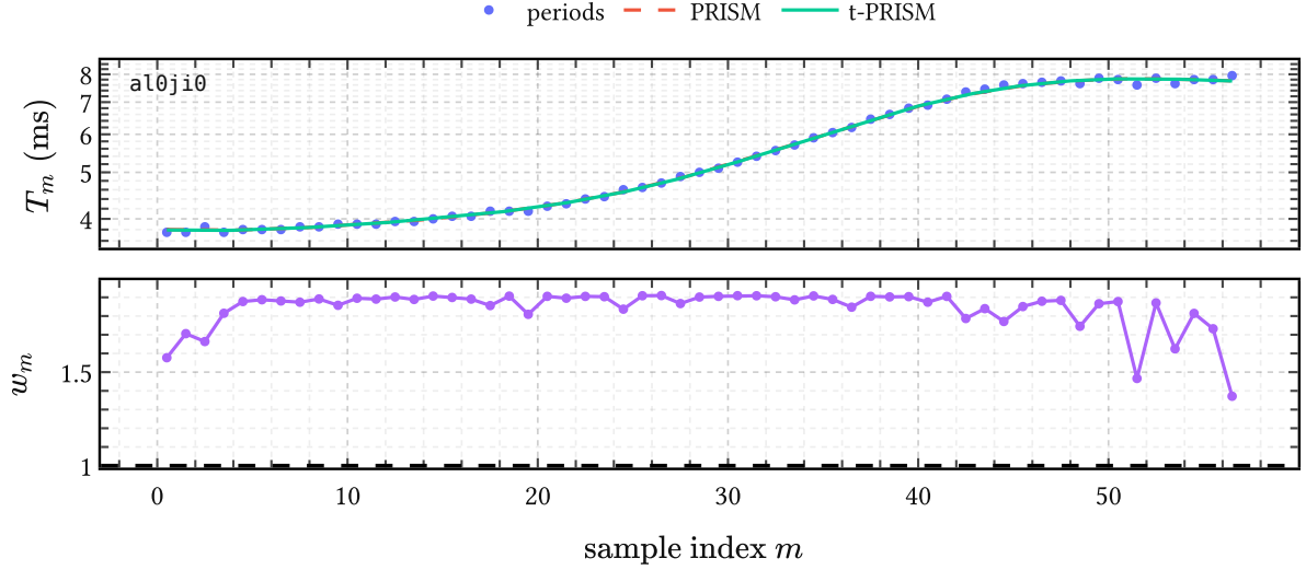
Figure 44 | t-PRISM reducing to PRISM in the absence of outliers. On this local APLAWD period track the observations are already consistent with a smooth trend. The PRISM and t-PRISM fits are nearly indistinguishable, and all inferred weights w_m \geq 1 and O(1) .
