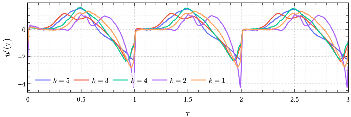
Figure 47 | Direct samples from the quantized manifold mixture in data space for the data in Figure 46. Here one first samples a component and manifold coordinate from q_K(\mathbf{x}) in (276), then pushes that sample through the GPLVM map described in Algorithm 4.5.2. and finally through the PRISM synthesis map (260) to Level 0. This shows the nonlinear generative mechanism itself, before moment matching replaces it by a Gaussian approximation in amplitude space.
