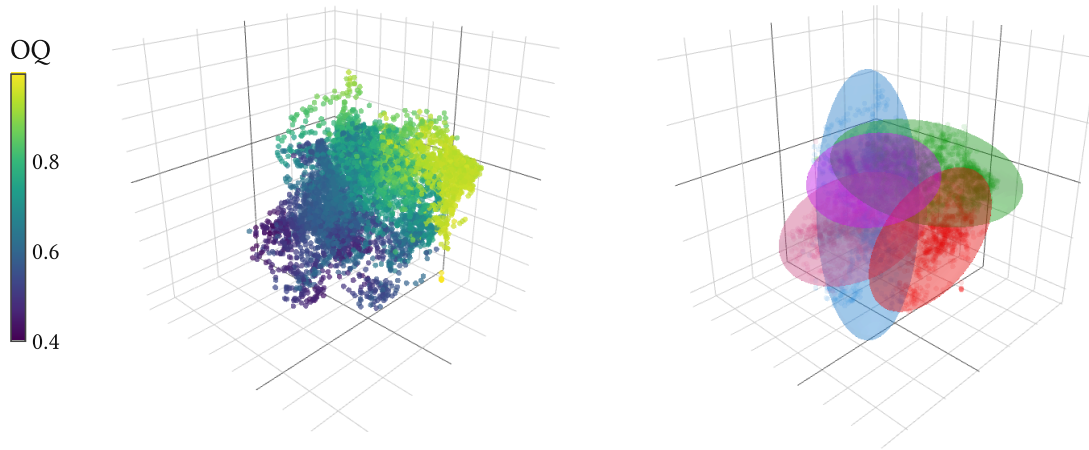
Figure 46 | Manifold structure and quantization on EGIFA. Left: the three-dimensional manifold space learned by q-GPLVM, with each waveform colored by open quotient. Right: the K = 5 fitted Gaussian ellipsoids used for quantization in that same manifold space (277). The left panel shows that open quotient varies smoothly over the manifold rather than appearing as disconnected clusters, while the right panel shows how XDGMM compresses the empirical mixture (275) into the K = 5 approximation q_K(\mathbf{x}) of (276).
