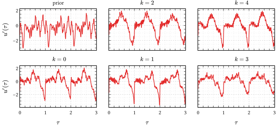
Figure 48 | Samples from the moment-matched prior in data space for the data in Figure 46. The “prior” panel at the top left draws from the PRISM prior (289), which are just generic combinations of the learned PRISM basis. The other panels condition on individual mixture components in (291) and have learned to model the density in amplitude space, each mixture component k modeling different types of DGF waveforms. Note how much more structured and DGF-like these are in comparison to the “prior” panel.
