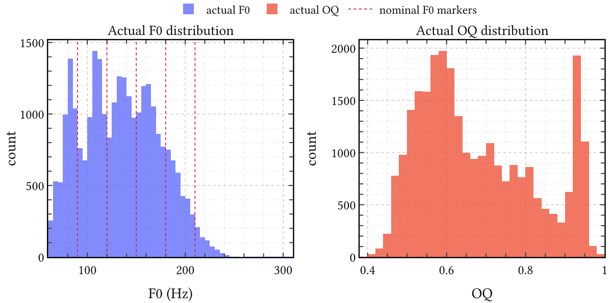
Figure 36 | Implied F_0 and OQ distributions from LBGID on EGIFA. Left: frame-level F_0 implied by detected GCIs, with dashed lines at EGIFA’s nominal pitch settings. Right: frame-level OQ implied by detected GCI/GOI pairs.
