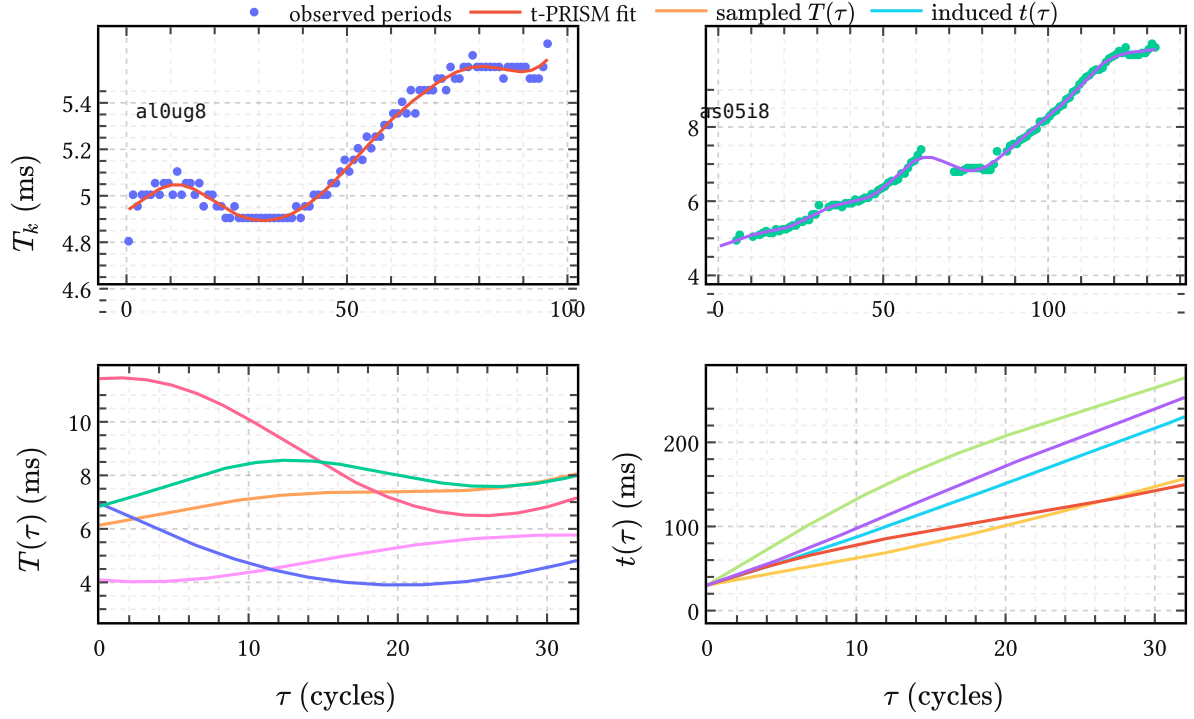
Figure 31 | From learned pitch prior to time warp. Top: two retained APLAWD period tracks together with their t-PRISM posterior means. Bottom left: prior samples of the instantaneous period function T(\tau) from the learned APLAWD model. Bottom right: the corresponding induced warps t(\tau) = t_0 + \int_0^\tau T(u) du . This is the object needed later to turn refined DGF surrogates in cycle time into voiced signals in physical time.
