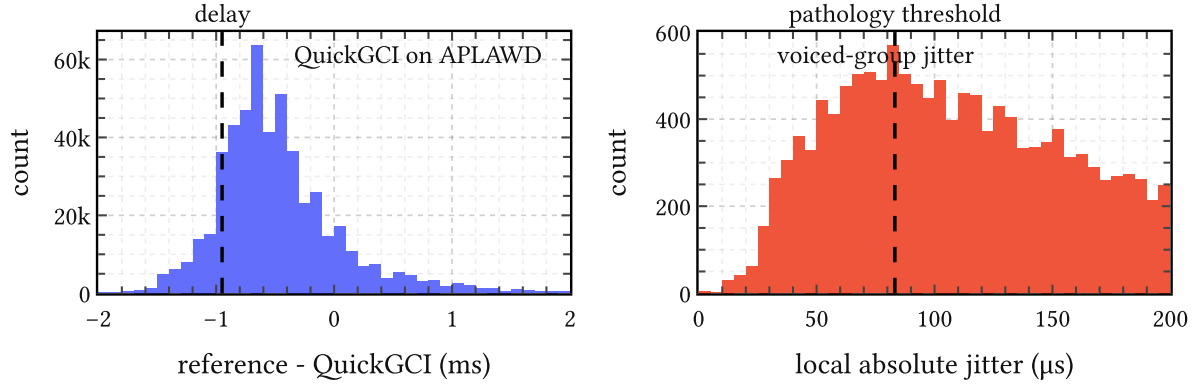
Figure 38 | Two APLAWD diagnostics. Left: QuickGCI timing errors against the hand-corrected GCI references. The mode is centered close to the expected larynx-to-microphone delay. Right: local absolute jitter measured over retained voiced groups. Most of the mass lies well below the usual pathology threshold.
