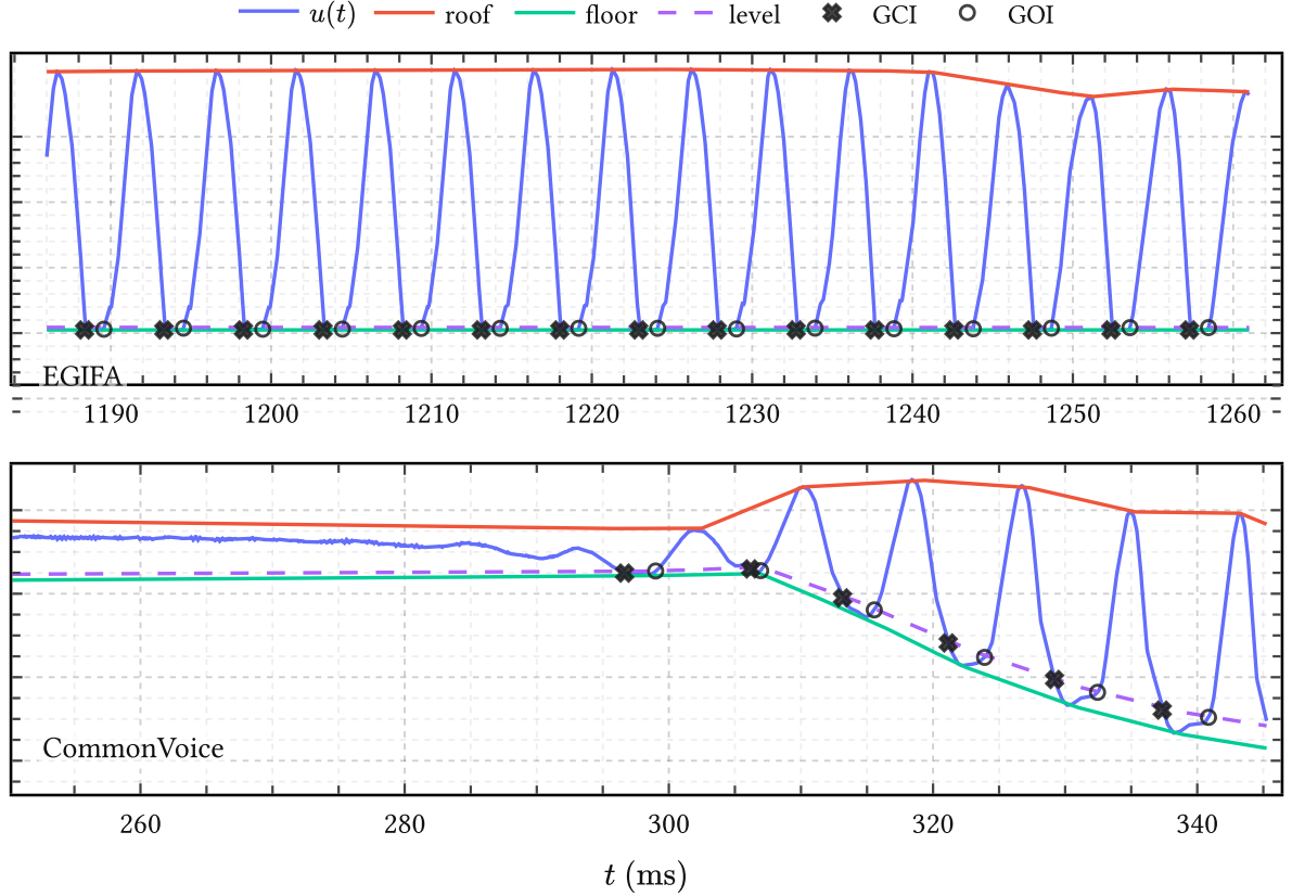
Figure 41 | LBGID on EGIFA and CommonVoice . Each panel shows u(t) together with \text{roof}(t) , \text{floor}(t) , the relative threshold \text{level}(t) , and the detected (GCI, GOI) pairs. On EGIFA we use \alpha = 0.01 ; on CommonVoice we use \alpha = 0.10 . Note how the level function rejects the non-voiced part (roughly before 300 ms) in the bottom panel.
