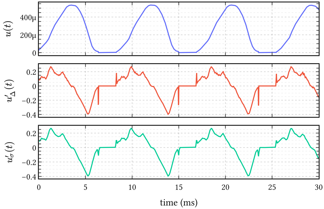
Figure 62 | Smooth differentiation dampens spikes in u'(t) . The top panel shows the ground truth glottal flow u(t) extracted from a random EGIFA file. The middle panel contains its derivative u'_\Delta(t) obtained by finite differences (345), and the bottom panel the Gaussian-smoothed derivative u'_\sigma(t) proposed in (346). It can be seen that raw differentiation amplifies sample-scale fluctuations into large spikes, whereas the smoothed derivative retains the closure structure at the intended temporal resolution.
