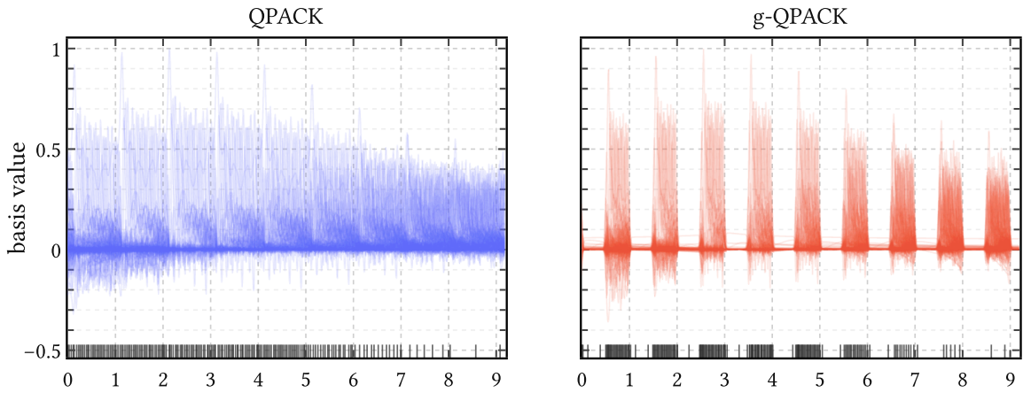
Figure 31 | Learned bases for the strongest matched QPACK and g-QPACK configurations. Left: the best QPACK restart within the pack:1, R=192, J=16 family. Right: the best g-QPACK restart within the same family. Each panel shows the learned basis functions \varphi(\tau) \in \mathbb{R}^R on a \tau -grid. The locations of the inducing points are also shown as a carpet plot.
