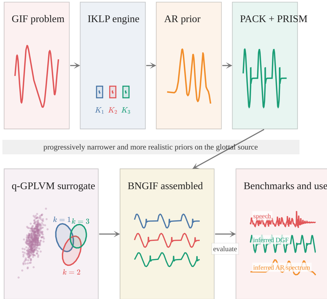
Figure 4 | The thesis as a sequence of prior refinements. Each step keeps the same voiced-speech inverse problem in view, but narrows the glottal source prior from a broad kernel bank to a compact surrogate that can finally be conditioned frame by frame in BNGIF.
