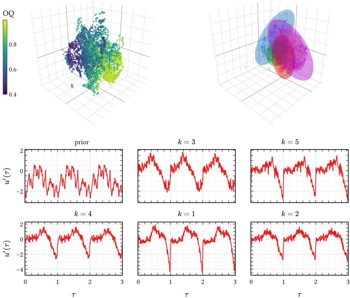
Figure 34 | QPACK surrogate: manifold space, quantization, and data-space samples. Top left: posterior means \{\mu_n^x\}_{n=1}^N from \mathcal{D}_Q , shown as a manifold point cloud and colored by ground-truth OQ. Top right: the K = 5 XDGMM ellipsoids of \mathcal{M}_Q fit to the data in the top left panel. Bottom: the left panel samples the unrefined PRISM prior p(\mathbf{u}' | \tau, \mathcal{D}_R) from (172); the numbered panels sample the k -th component conditionals of p(\mathbf{u}' | \tau, \mathcal{M}_R) induced by (173).
