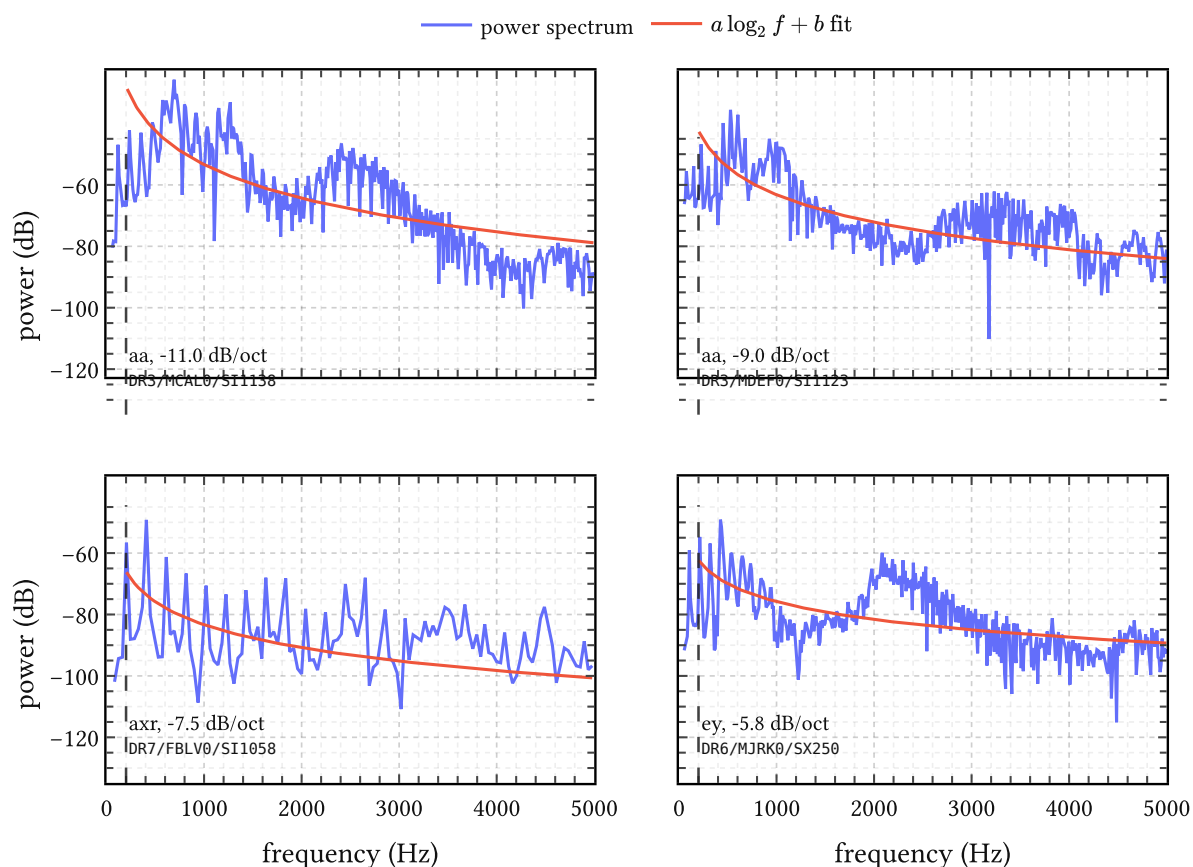
Figure 53 | Example spectral-tilt fits on retained TIMIT vowel events. Each panel shows the empirical power spectrum together with the fitted trend a \log_2 f + b . The dashed vertical line marks the 200 Hz cutoff above which the fit is performed. This is a supporting estimate derived from the same TIMIT/VTR pairing, not the main benchmark object of the chapter.
