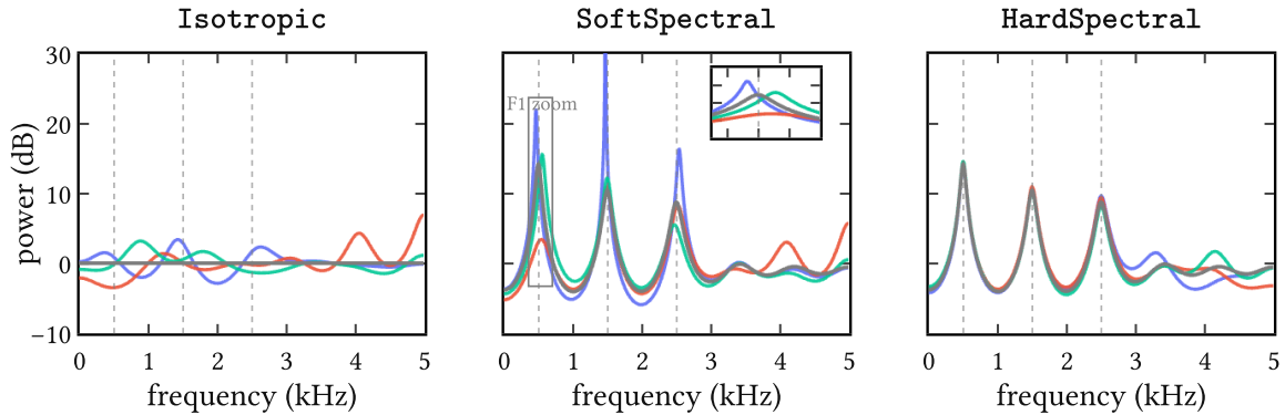
Figure 13 | Example of imposing spectral features on an isotropic base prior leading to the soft and hard spectral shaping priors from (57) and (60). We used a constraint polynomial M(z) = Q_1(z) \cdot Q_2(z) \cdot Q_3(z) to encode the spectral features for this example. These are three resonances at (F_1, F_2, F_3) = (500, 1500, 2500) Hz as indicated by the dashed vertical lines. Each panel shows the spectrum mean (grey) together with three samples (colors) of the associated prior. From left to right, these are (1) the base prior p_0(\mathbf{a}) := \text{Isotropic}(0.1/P) with P = 12 ; (2) the soft spectral shaping prior \text{SoftSpectral}(\mathbf{0}, (0.1/P)\mathbf{I}_P; M) with an inset that zooms in on the F_1 region; and (3) the hard spectral shaping prior \text{HardSpectral}(\mathbf{0}, (0.1/P)\mathbf{I}_P; M) .
