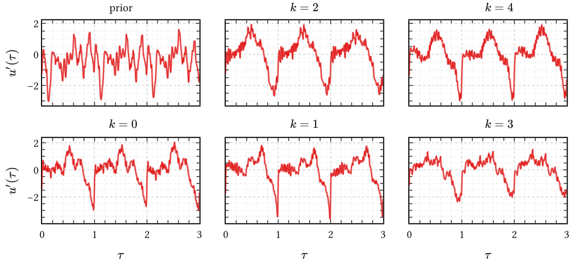
Figure 43 | Samples from the moment-matched prior in data space. The prior panel draws from the full mixture (279), while the other panels condition on individual mixture components. Compared with Figure 42, this is the Gaussian approximation actually retained by the thesis: the nonlinear push-forward has been summarized by moment matching in amplitude space and then synthesized back to Level 0.
