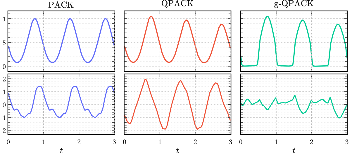
Figure 21 | From PACK to QPACK to g-QPACK. The top row shows kernel sections at anchor time t' = 0.75 and the bottom row prior samples, all with matched carrier hyperparameters. QPACK relaxes strict periodicity by adding a slow envelope and baseline; g-QPACK then suppresses covariance in the less informative phase of the cycle. The shared carrier settings are d = 1 , J = 1 , T = 1 , and w = (0.2, 0.8) ; the QPACK envelope and baseline are the same as in Figure 20, and the gate sharpness of g-QPACK is \alpha = 12 .
