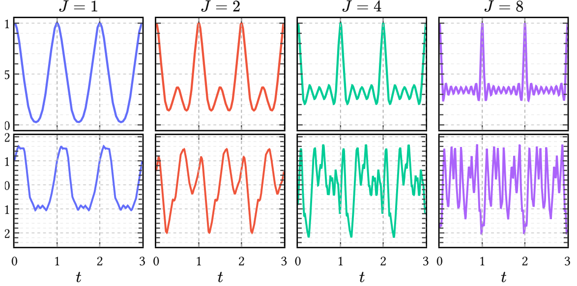
Figure 18 | Effect of harmonic order J on PACK. The top row shows the kernel section k(t, 0) and the bottom row a prior sample. At fixed degree d = 1 , increasing J decreases the effective within-cycle lengthscale and yields progressively wigglier covariance structure and sample paths. The remaining hyperparameters are fixed at T = 1 , \sigma_a^2 = 1 , w_0 = 0.2 , and uniform harmonic weights w_1, \dots, w_J over the remaining mass.
