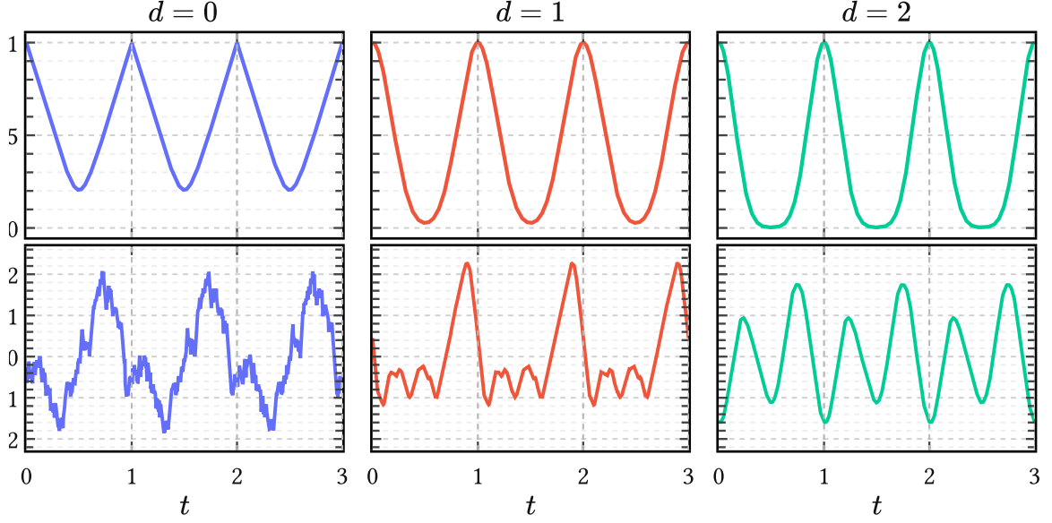
Figure 19 | Effect of degree d on within-cycle smoothness. The top row shows the kernel section k(t, 0) and the bottom row a prior sample. Holding J and the harmonic weights fixed, increasing d softens the changepoint-like geometry and produces smoother periodized waveforms. The remaining hyperparameters are fixed at J = 1 , T = 1 , \sigma_a^2 = 1 , w_0 = 0.2 , and w_1 = 0.8 .
