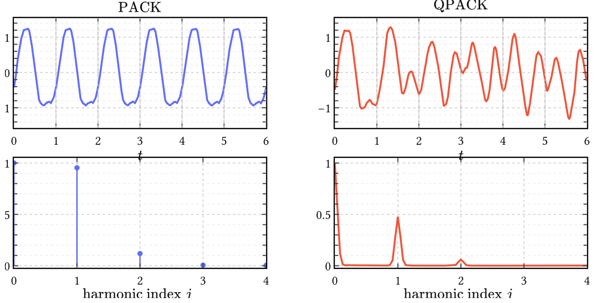
Figure 20 | From PACK to QPACK in time and frequency. The top row shows prior samples over six periods; the bottom row shows the corresponding normalized spectra. PACK has a true line spectrum, whereas QPACK broadens these lines through slow envelope modulation and adds low-frequency mass through the baseline term. The shared carrier hyperparameters are d = 1 , J = 1 , T = 1 , \sigma_a^2 = 1 , and w = (0.2, 0.8) . For QPACK the envelope is an RBF kernel with lengthscale 4, and the baseline is a rational quadratic kernel with variance 0.05, lengthscale 0.12, and \alpha = 1 .
