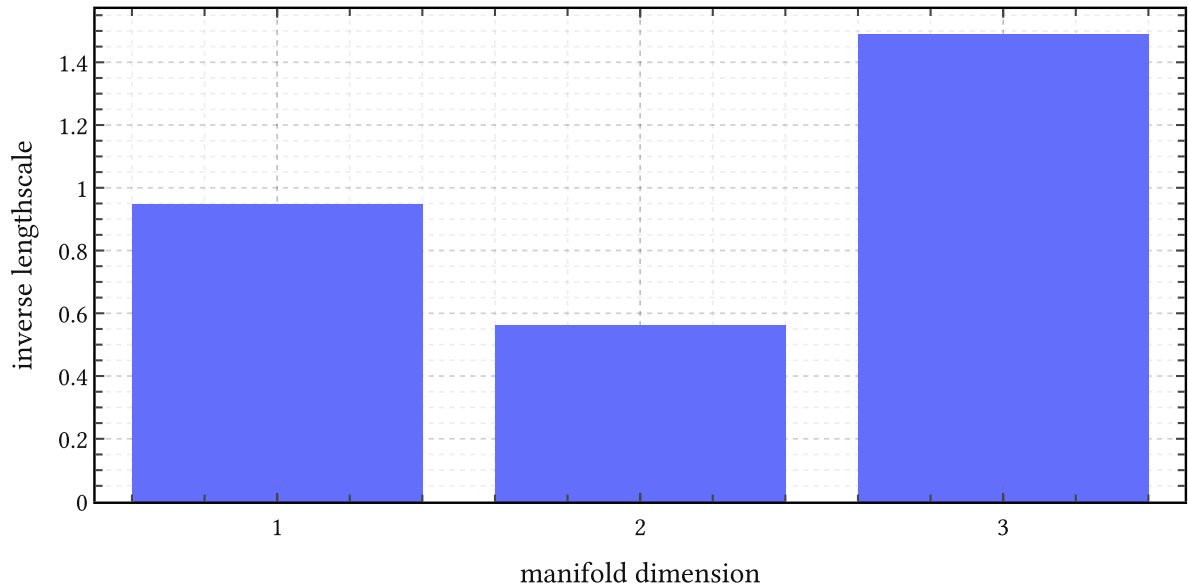
Figure 40 | Inverse lengthscales in manifold space. The ARD kernel keeps all three manifold dimensions active on EGIFA, but not equally so. Larger inverse lengthscale means that the GPLVM map varies more strongly along that coordinate, so the third manifold dimension carries the sharpest structure while the second is the smoothest.
