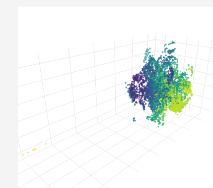
embedded corpus; each point is a glottal wave
