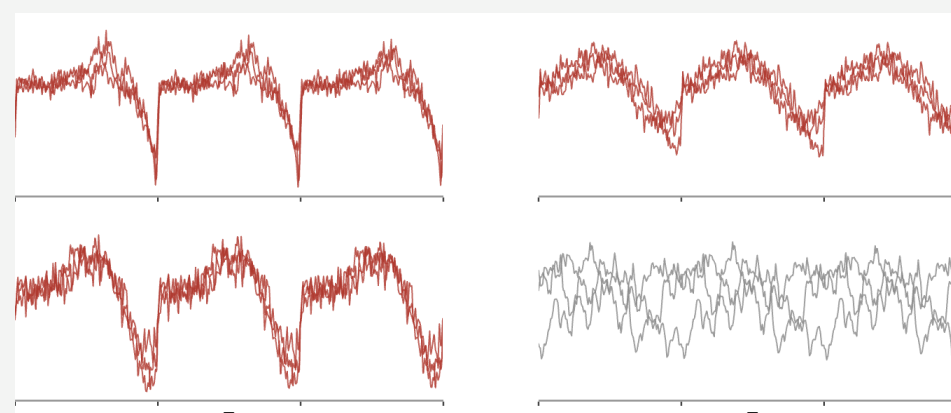
large corpus of glottal waves
