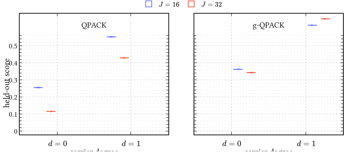
Figure 29 | Held-out calibration scores on EGIFA. Each box summarizes 32 independent PRISM initializations for a fixed carrier degree and harmonic order, using 128 inducing basis functions, an RBF envelope, and a rational quadratic baseline. The vertical axis reports mean held-out reduced-rank log evidence per effective sample on 500 test groups. All shown models lie far above their matched white-kernel nulls, omitted for readability. Gating shifts the entire score distribution upward, while harmonic order 16 is consistently more reliable than harmonic order 32 at fixed basis size.
