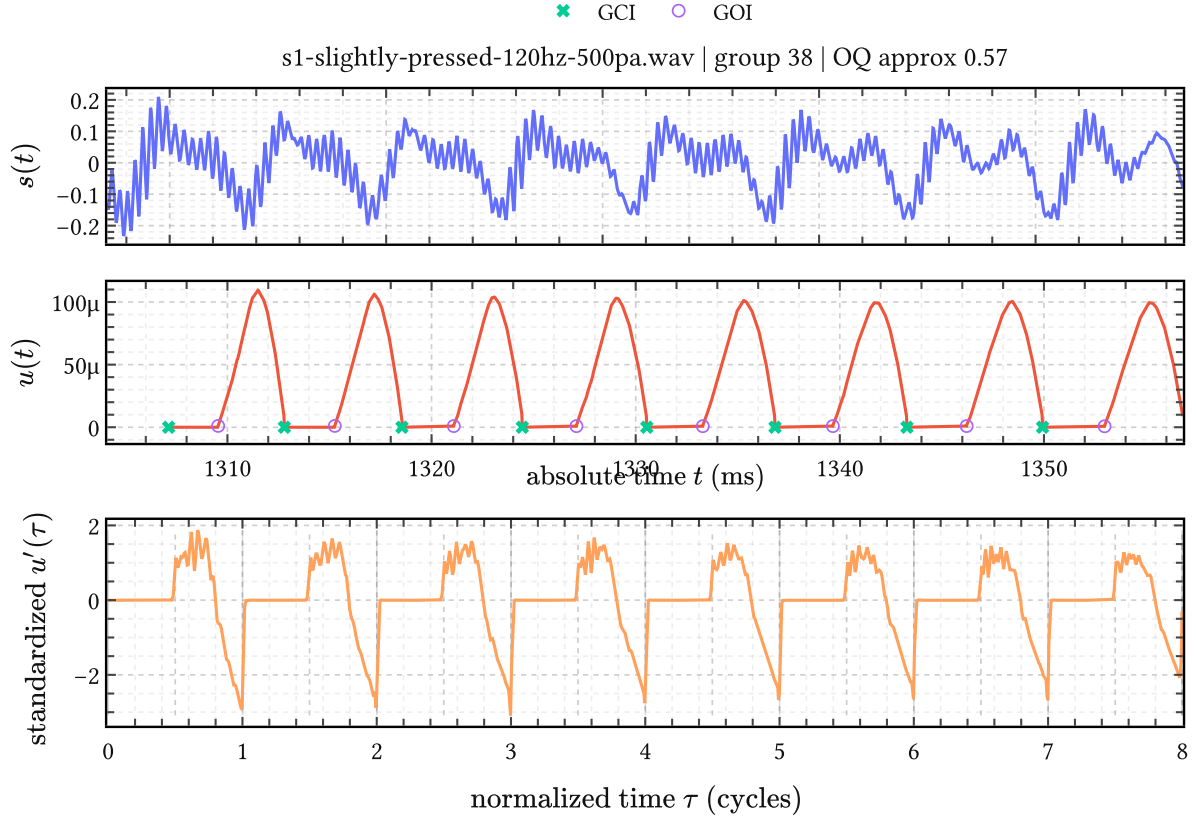
Figure 23 | Registration of one retained EGIFA voiced group. Top: the raw speech waveform s(t) in physical time. Middle: the corresponding raw glottal flow u(t) , again in physical time, with LBGID-detected GCI and GOI landmarks. Bottom: the same group after GOI-aware registration to shared cycle time, Gaussian smoothing, differentiation, and per-group standardization, now shown as u'(\tau) . In this representation the GCIs land at integers and the GOIs at half-integers, which is exactly the coordinate system needed by the later PACK-family calibration experiments.
