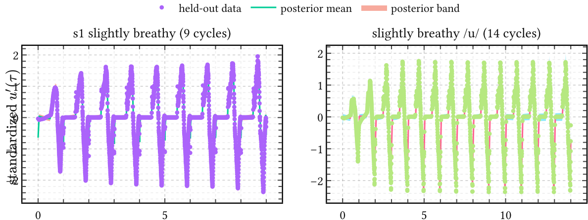
Figure 28 | Held-out fits from calibrated g-QPACK on EGIFA. Two retained EGIFA groups are shown together with posterior means and uncertainty bands from the best single held-out g-QPACK run (pack:2, J = 16 , M = 128 ). The shaded half-cycles [n, n + 1/2] indicate the phase registered as closed. After GOI registration, gating leaves these intervals comparatively de-emphasized while retaining flexible interpolation across the informative open phase.
